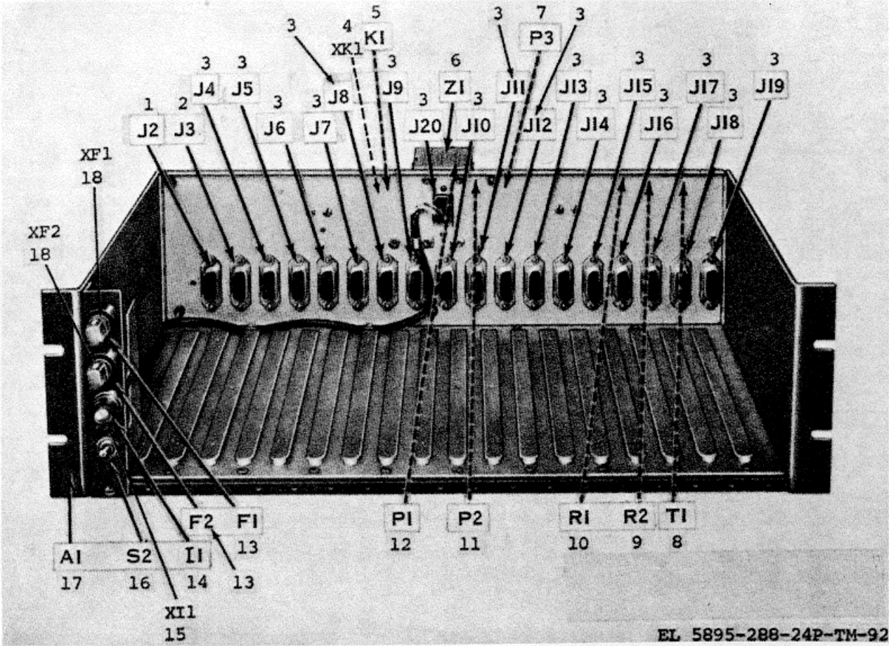
Figure 92. Tone Keyer Shelf, Type 221, Model 1
