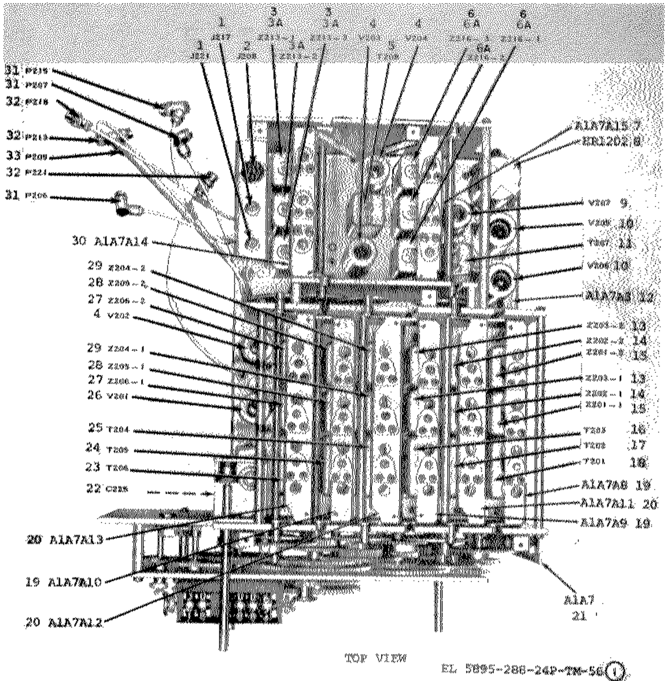
Figure 56. Radio Frequency Amplifier A1A7 (Sheet 1 of 3)
