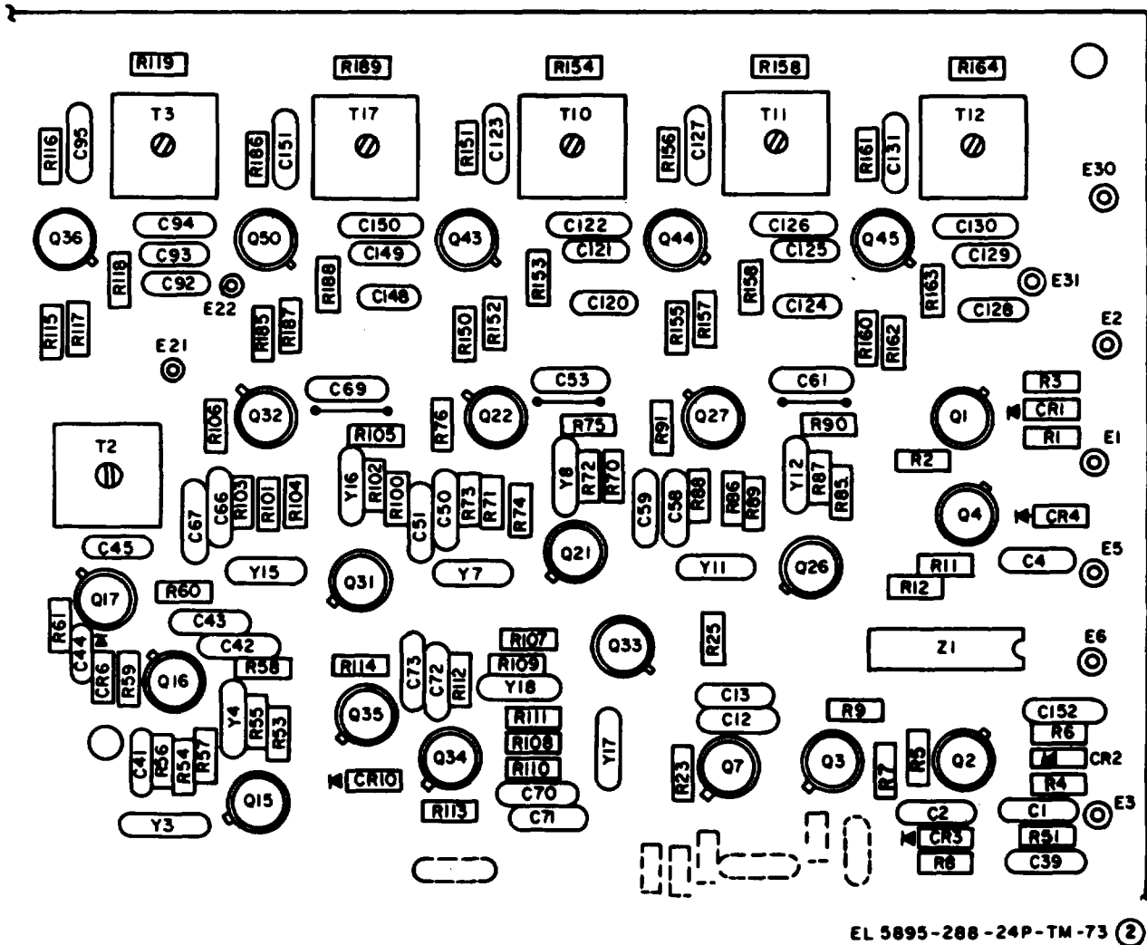
Figure 73. Spectrum Generator Circuit Card Z102 (Sheet 2 of 4)
