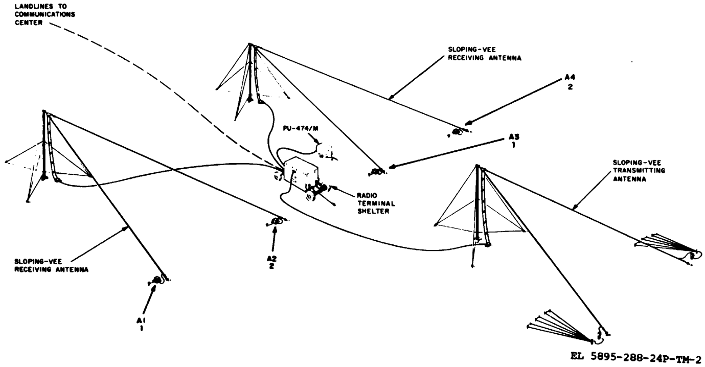
Figure 2. High Frequency Antenna System
