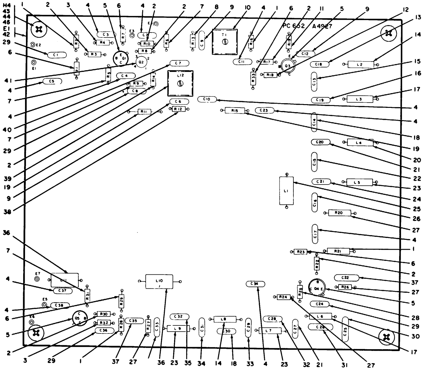
Figure 72. Second Mixer Circuit Card Z107
