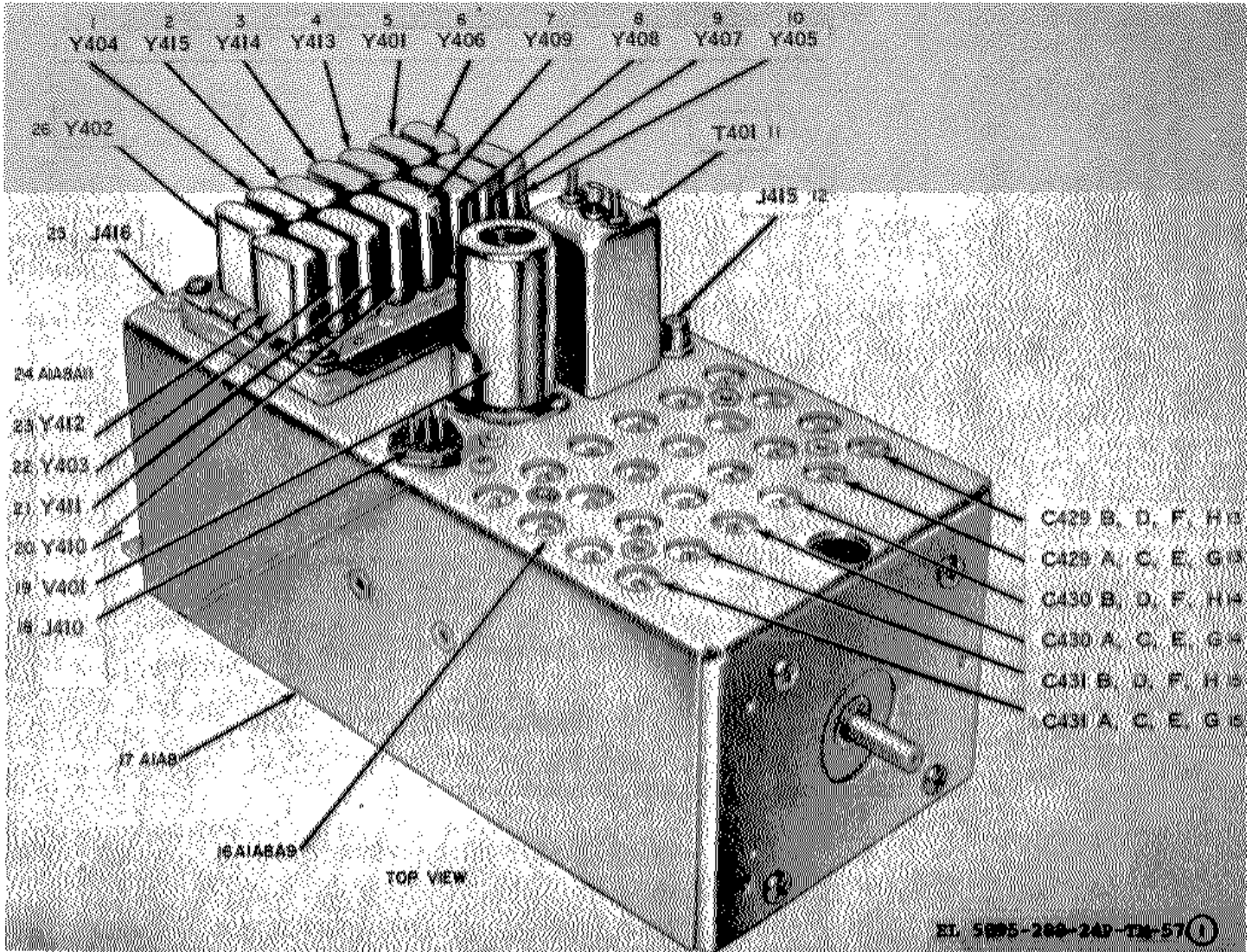
Figure 57. Crystal Oscillator Subchassis A1A8 (Sheet 1 of 3)
