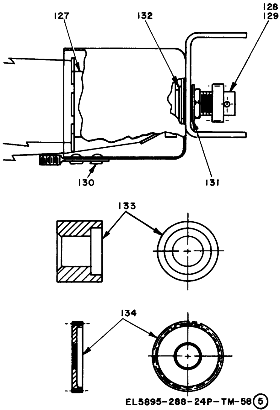
Figure 58. Gear Train Assembly A1A9 (Sheet 5 of 6)
