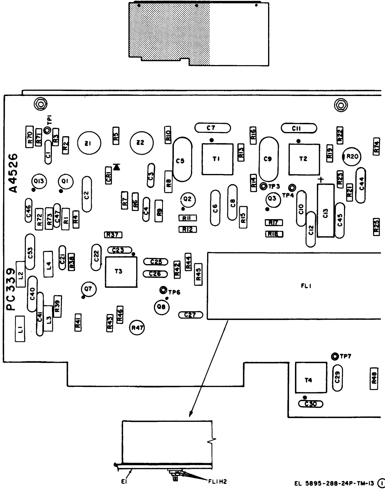
Figure 13. Carrier Generator Circuit Card Z109 (Sheet 1 of 2)
