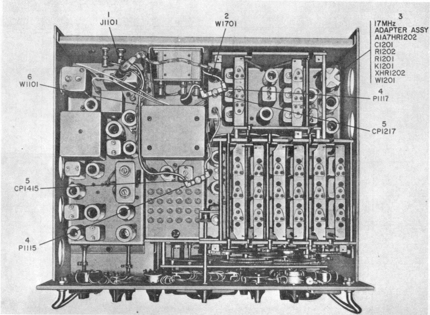
Figure 63. Radio Receiver Modification (Sheet 1 of 3)
