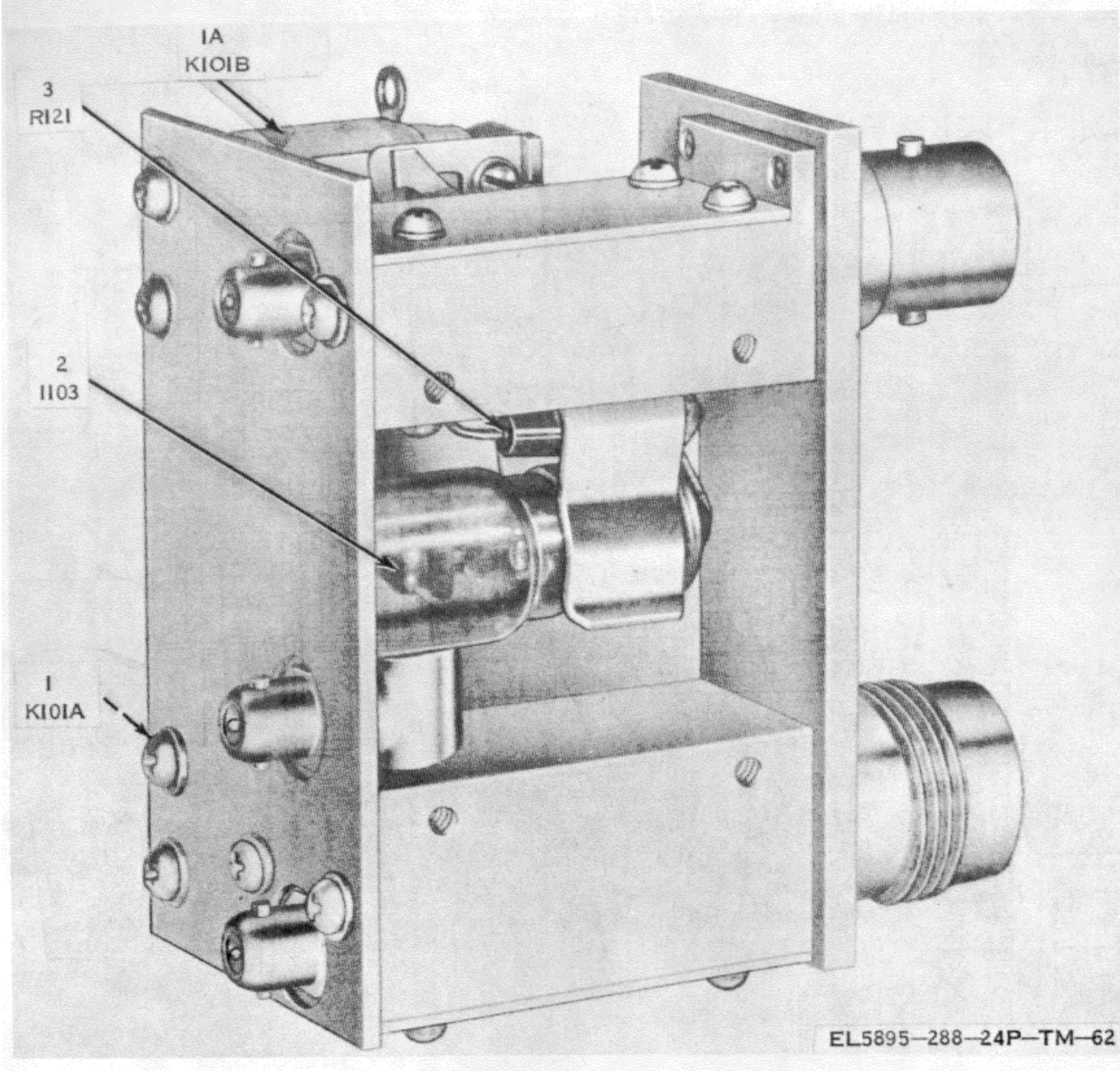
Figure 62. Antenna Relay Assembly
