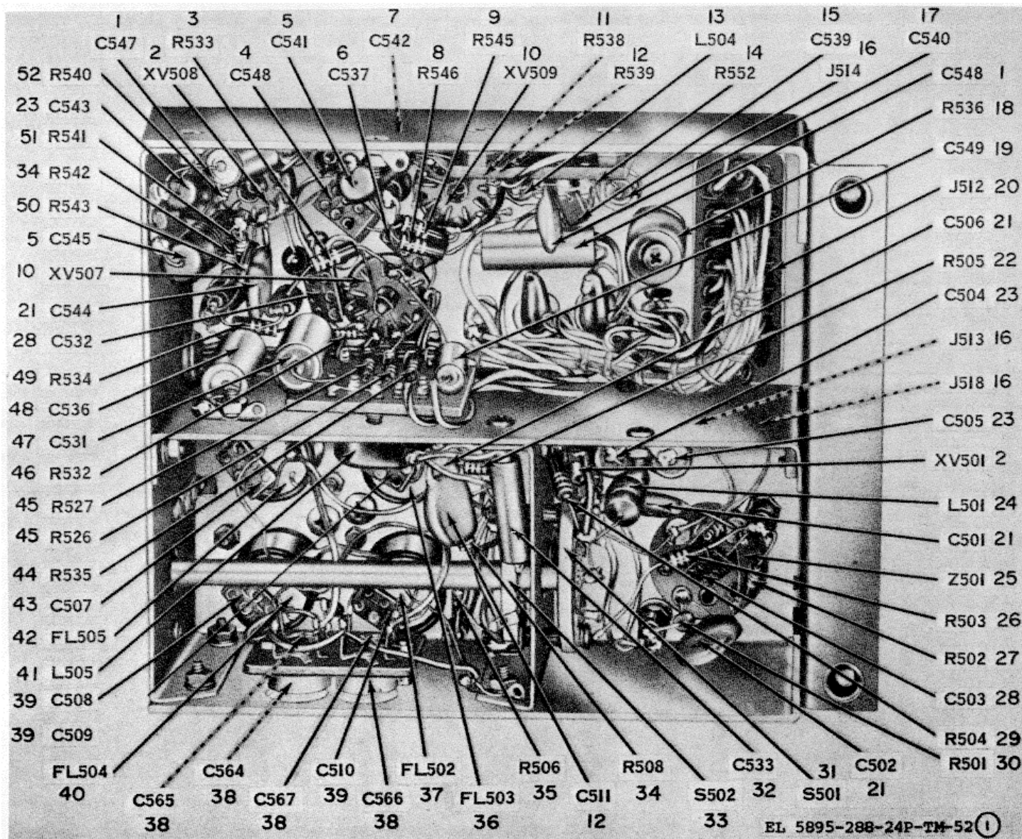
Figure 52. Amplifier subassembly, Bottom view Front Section (Sheet 1 of 2)
