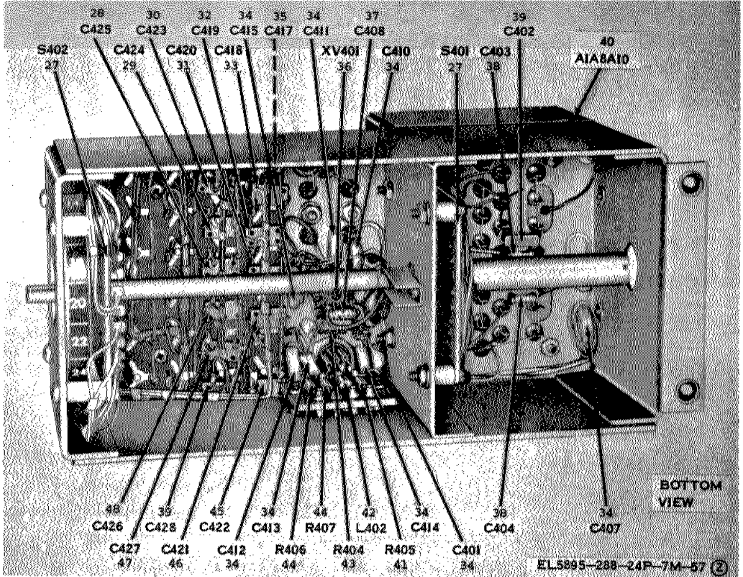
Figure 57. Crystal Oscillator Subchassis A1A8 (Sheet 2 of 3)
