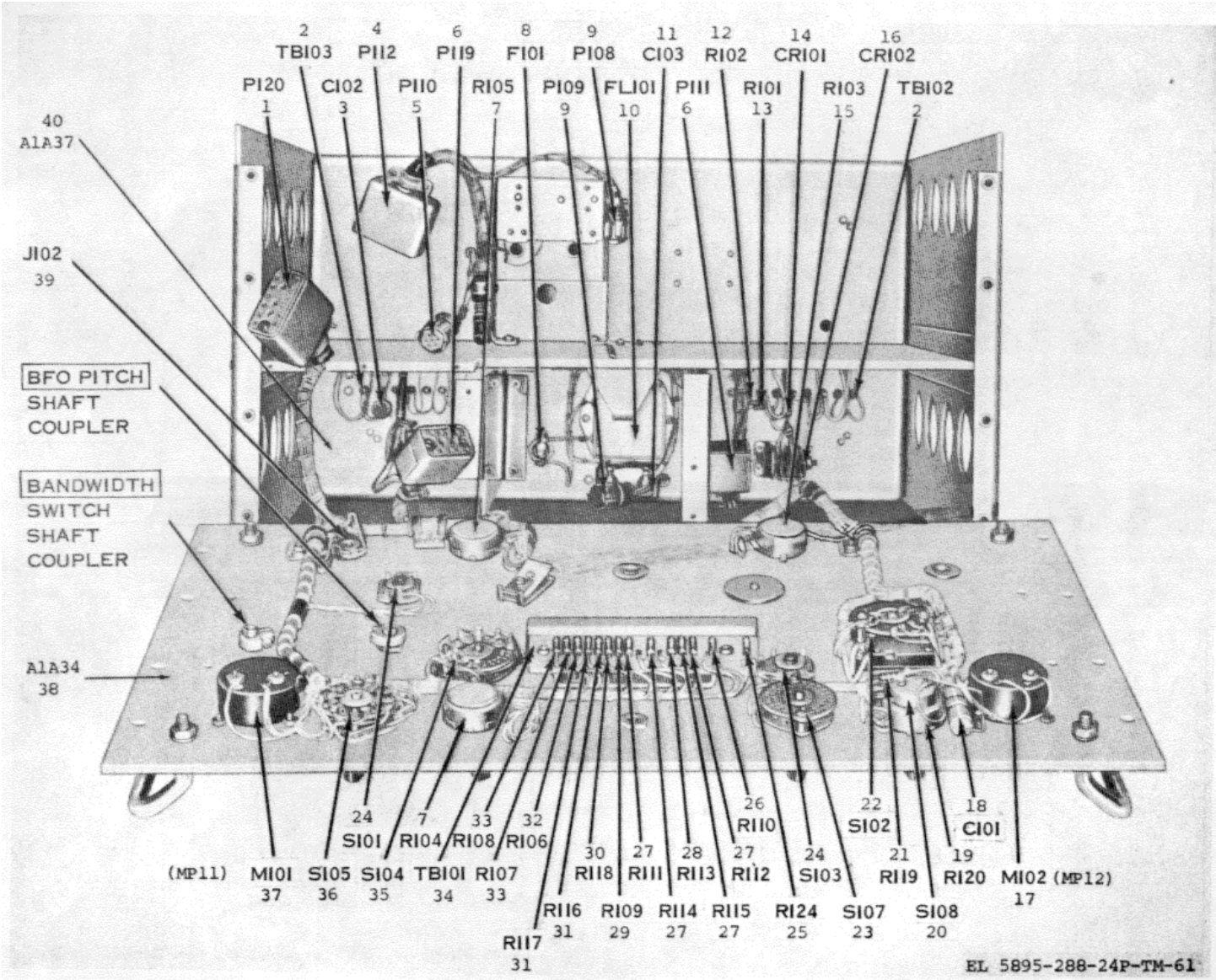
Figure 61. Front Panel Assembly A1A34 and Main Frame
