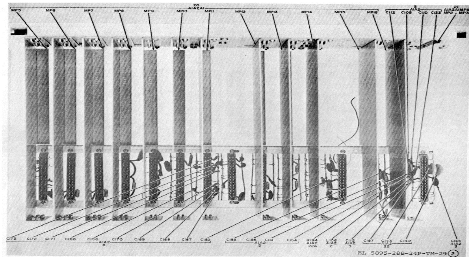
Figure 29. Multimode Exciter Subassembly A1A2 (Sheet 2 of 6)
