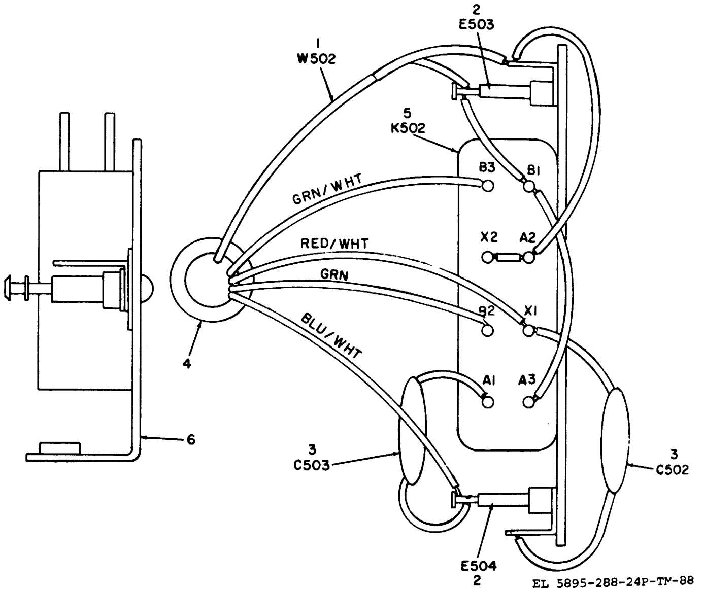
Figure 88. 555 KHz Oscillator Modification
