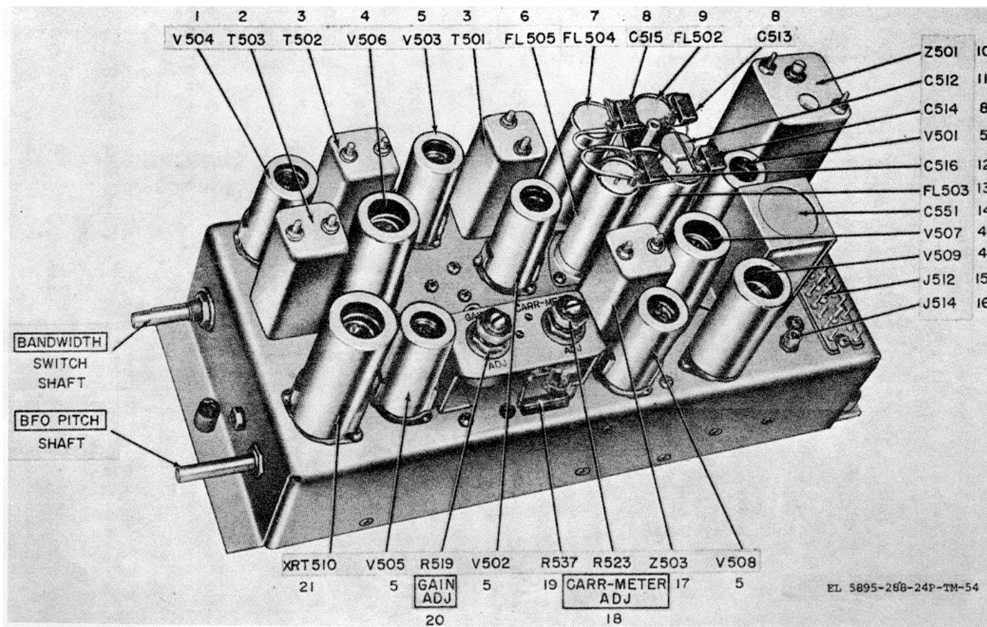
Figure 54. Unmodified IF Subchassis, Top View
