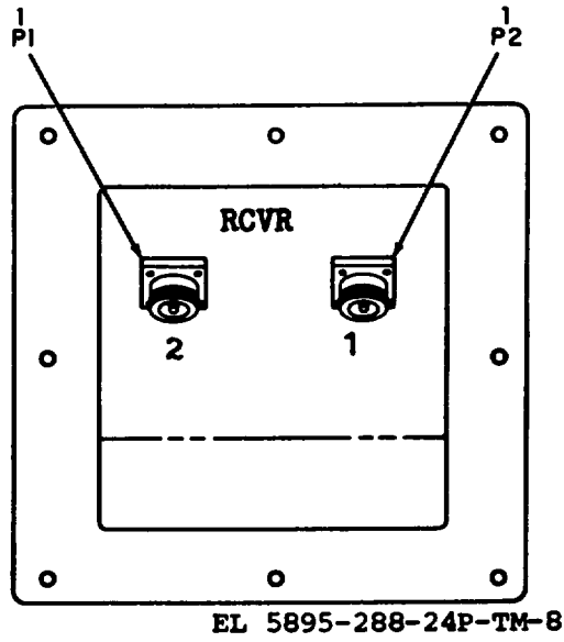
Figure 8. HF Receiving Entrance Box
