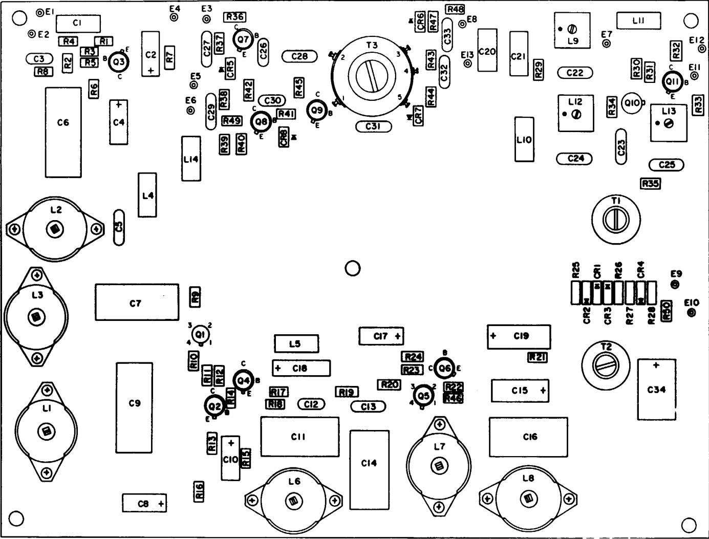
Figure 69. 10 and 100 kHz Multiplier Circuit Card Z108
