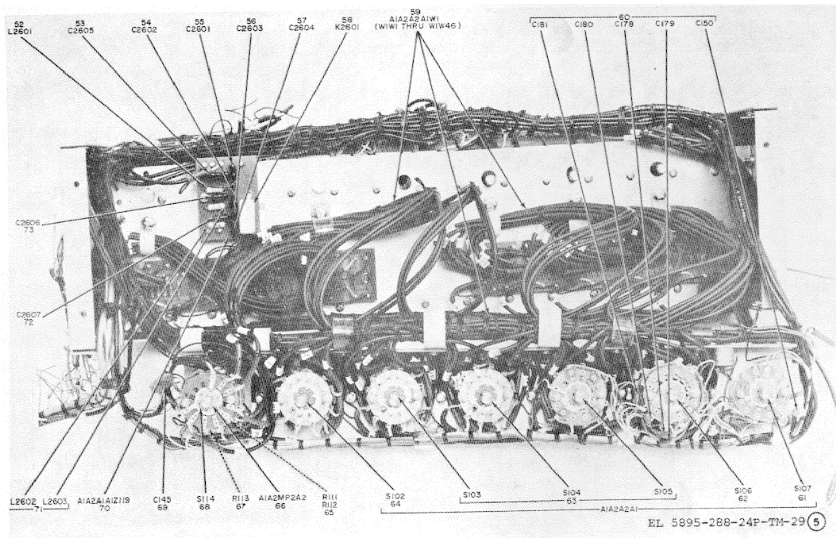
Figure 29. Multimode Exciter Subassembly A1A2 (Sheet 5 of 6)
