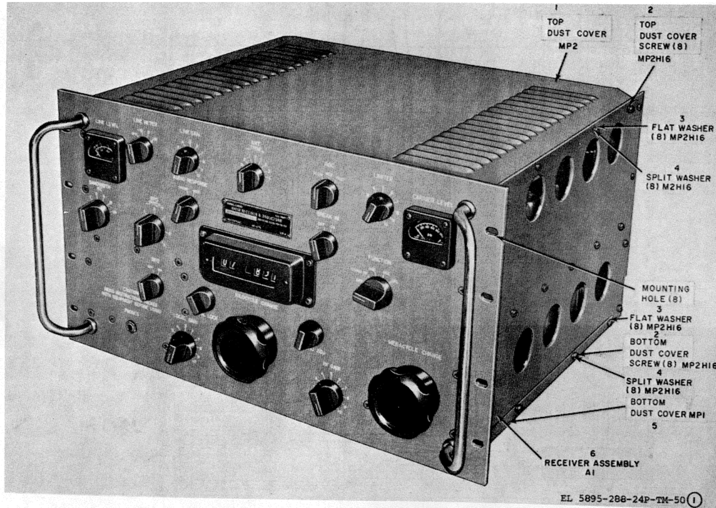
Figure 50. Radio Receiver P-1981/TSC-25 (Sheet 1 of 3)
