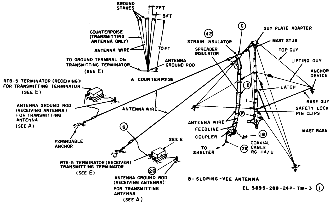
Figure 3. Antenna Mast- AB-746/G (Sheet 1 of 4)
