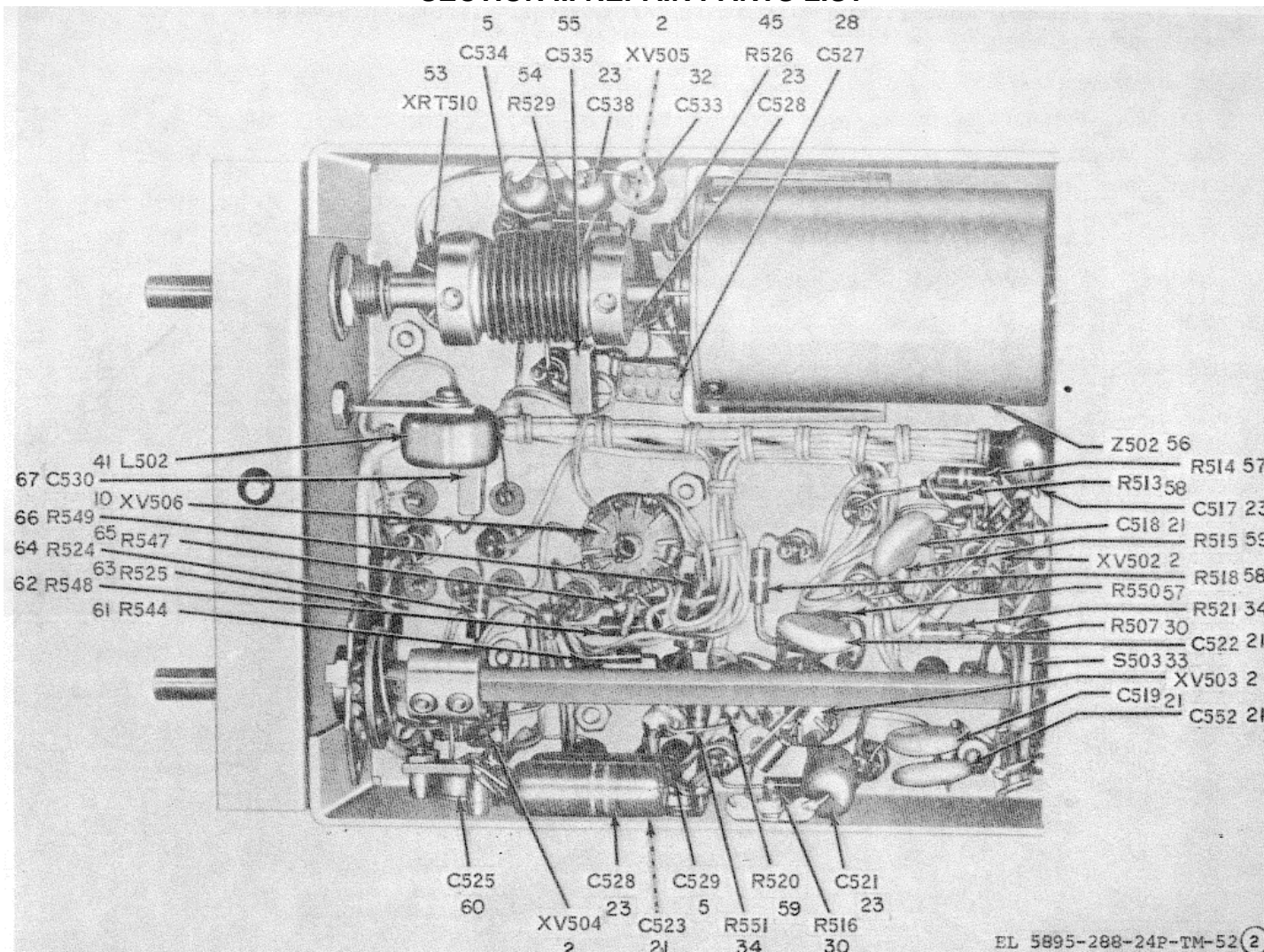
Figure 52. Amplifier Subassembly, Bottom View Front Section (Sheet 2 of 2)
