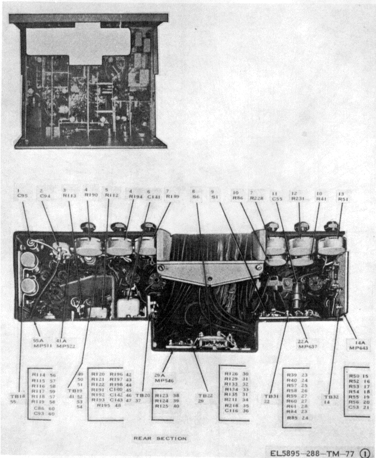
Figure 77. Converter Drawer Assembly, Bottom View (Sheet 1 of 4)
