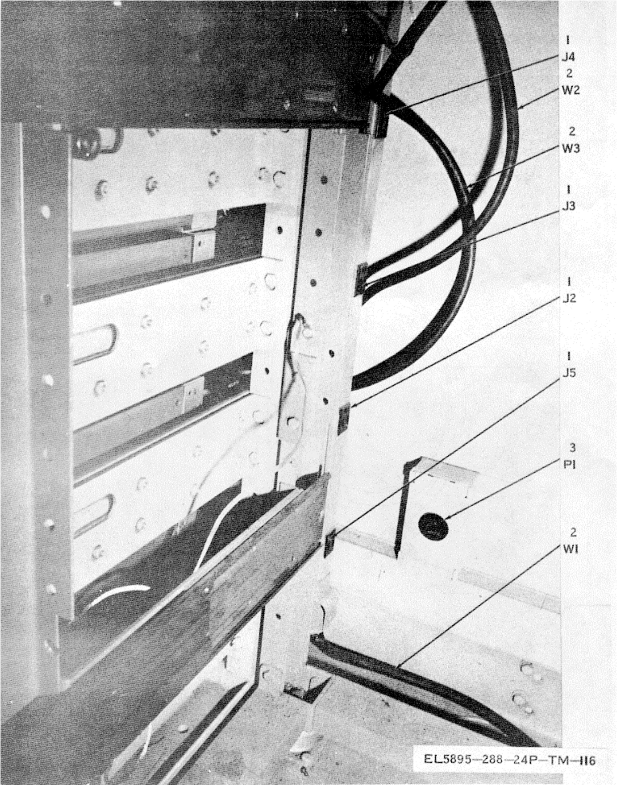
Figure 116. Power Cable Assemblies
