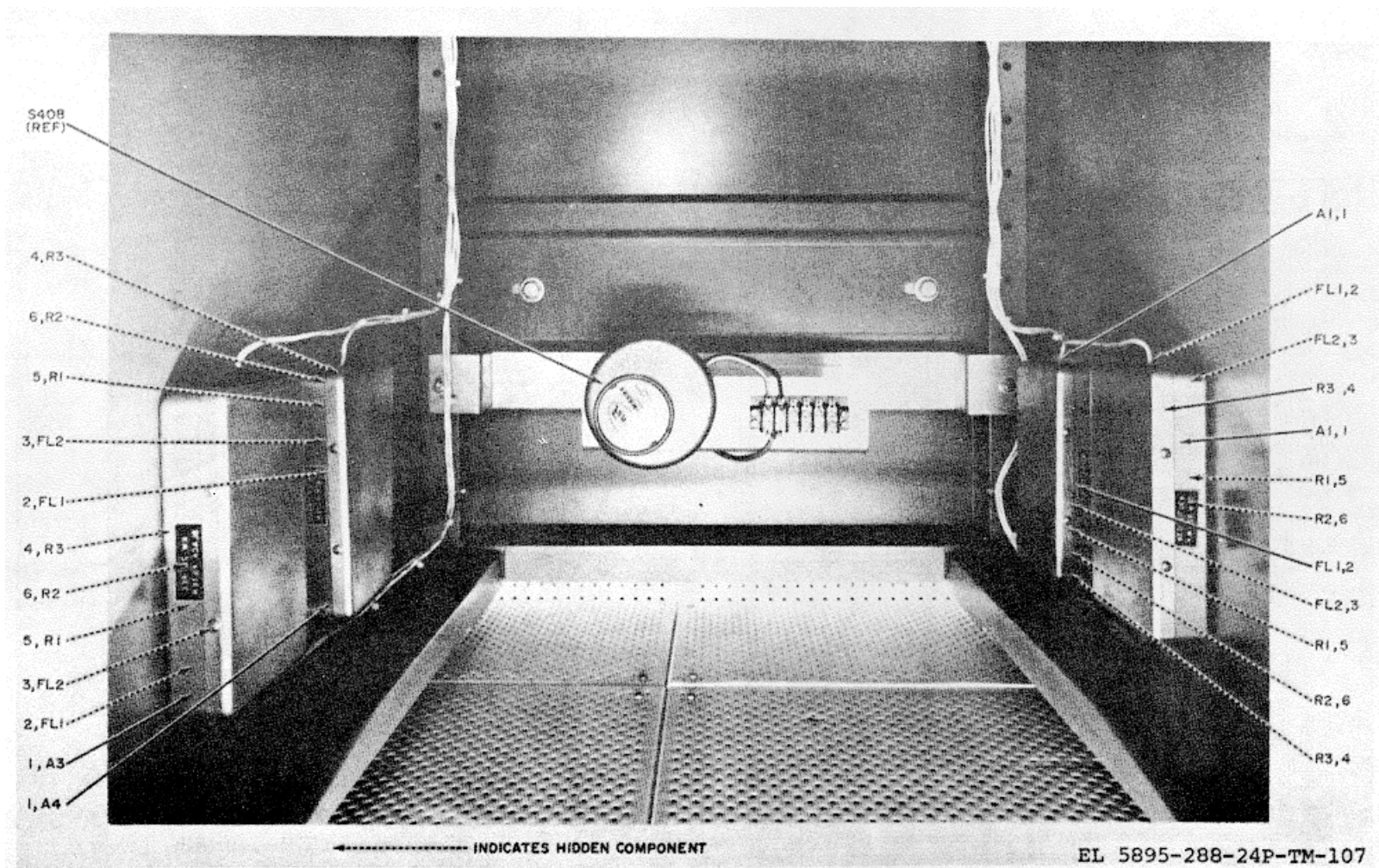
Figure 107. Installation Kit For TSEC/KW-26
