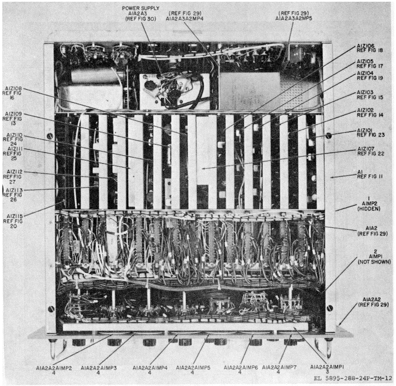
Figure 12. Multimode Exciter BMA-106
