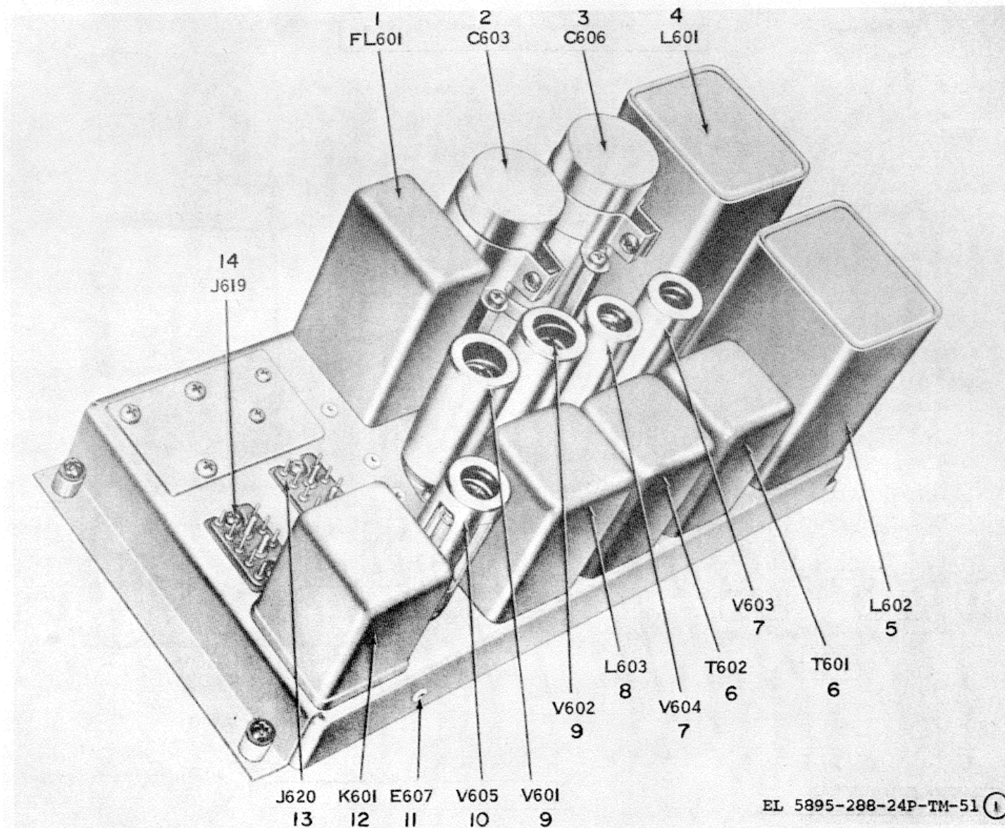
Figure 51. Audio Assembly A1A2 (Sheet 1 of 2)
