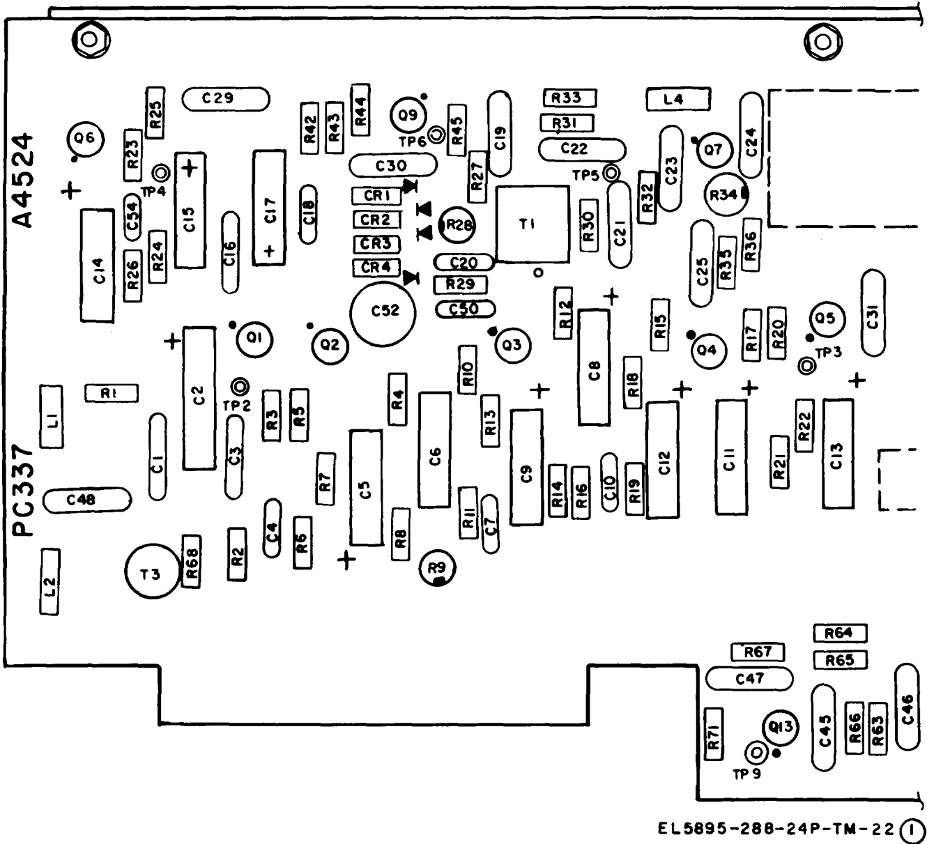
Figure 22. Sideband Generator Circuit Card Z107 (Sheet 1 of 2)
