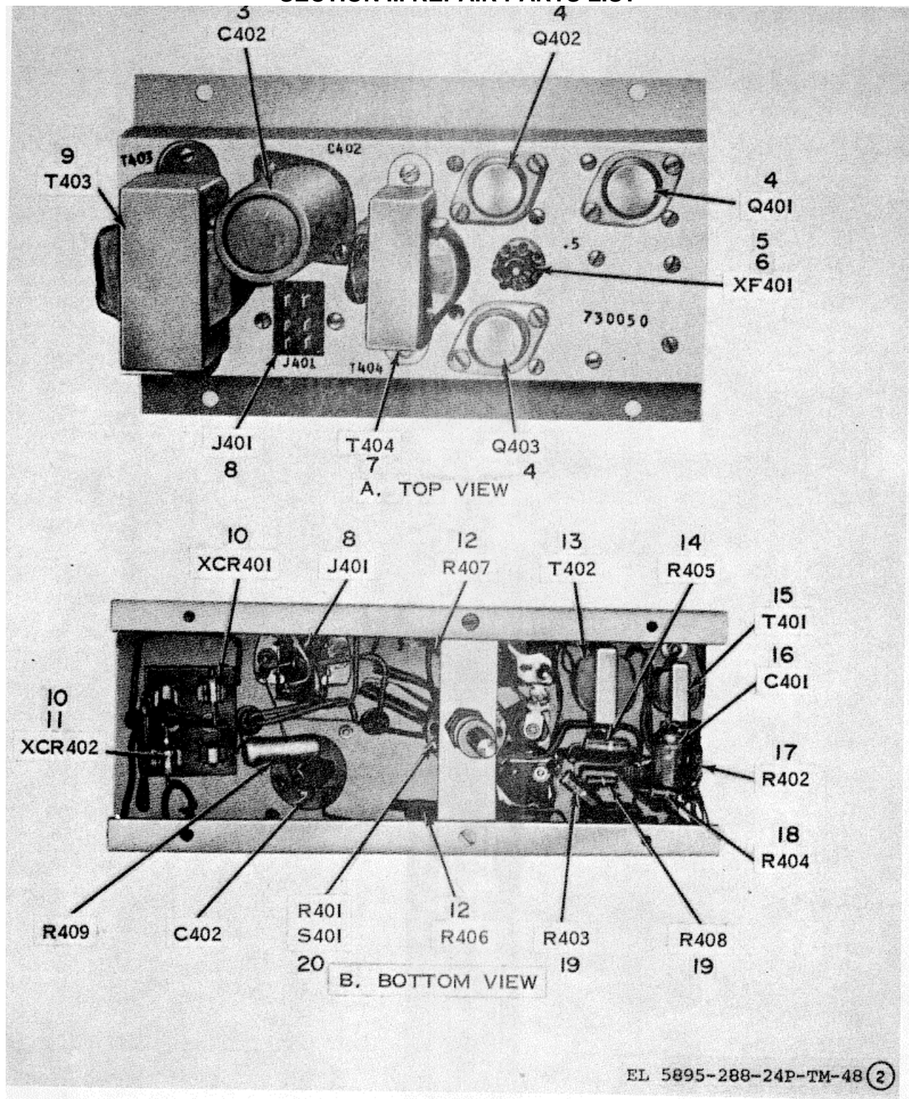
Figure 48. Dual Speaker and Amplifier Panel, Type 414A (Sheet 2 of 2)
