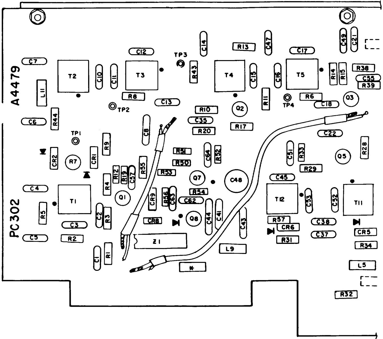
Figure 18. Mixer Divider Circuit Card Z106 (Sheet 1 of 2)
