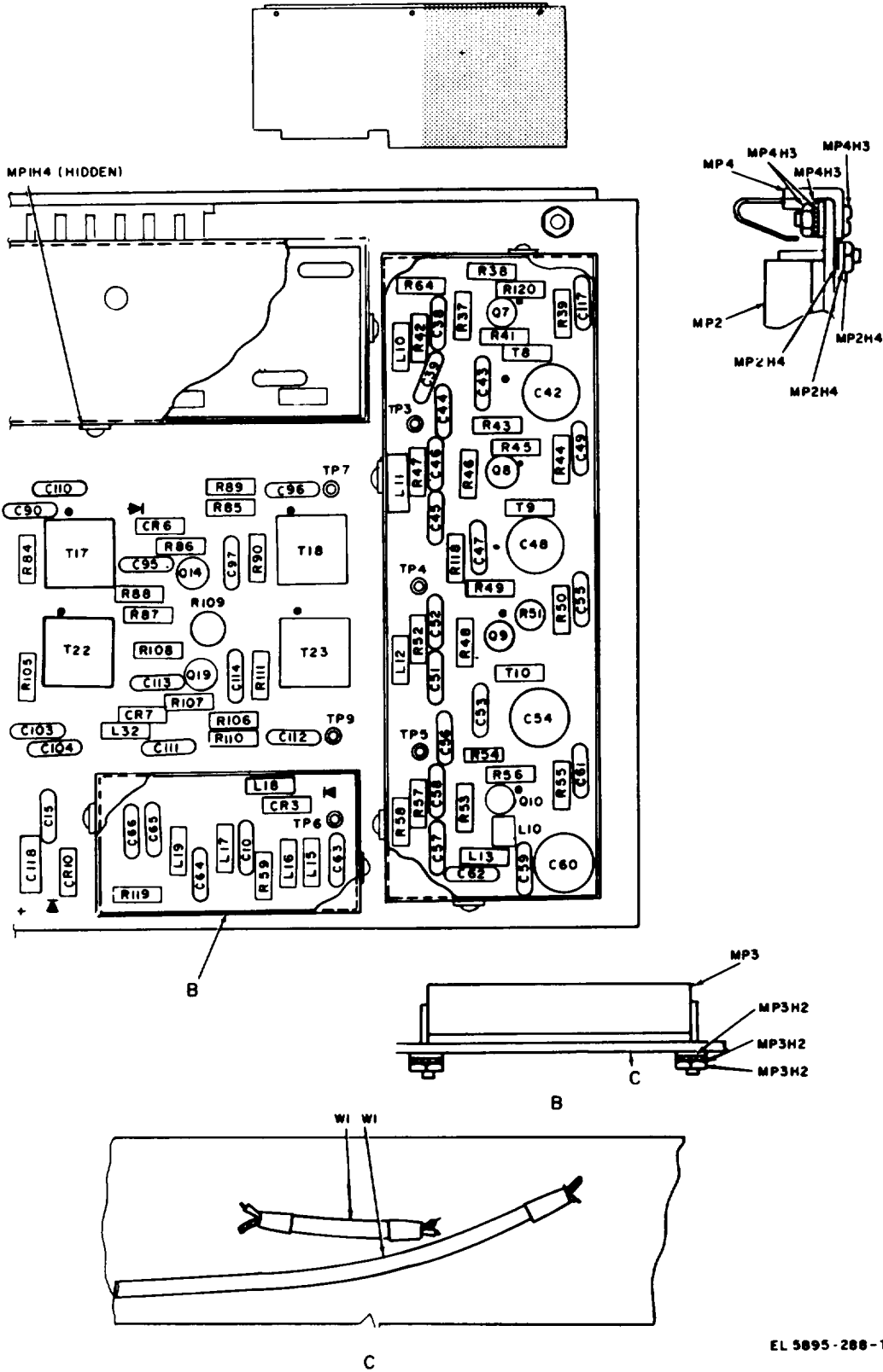
Figure 27. Translator Circuit Card z112 (Sheet 2 of 2)
