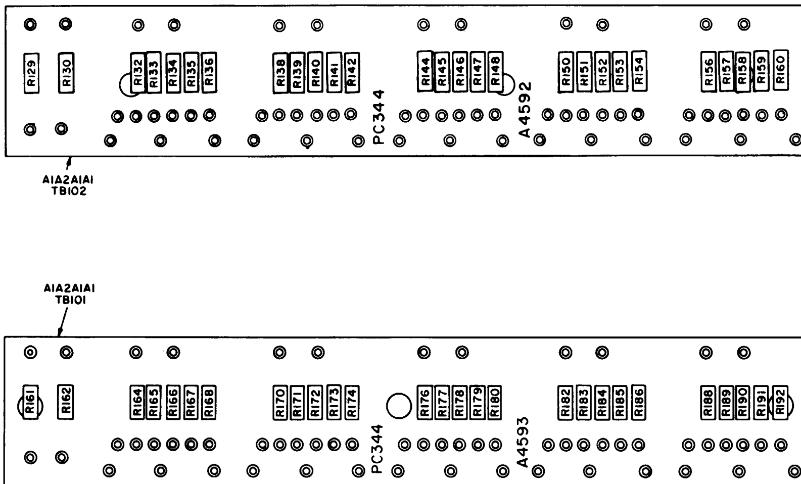
Figure 29. Multimode Exciter Subassembly A1A2 (Sheet 4 of 6)
