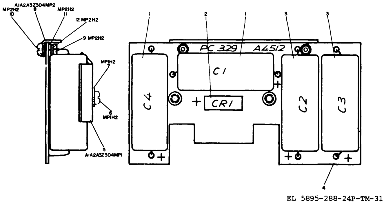
Figure 31. Circuit Card A Z304
