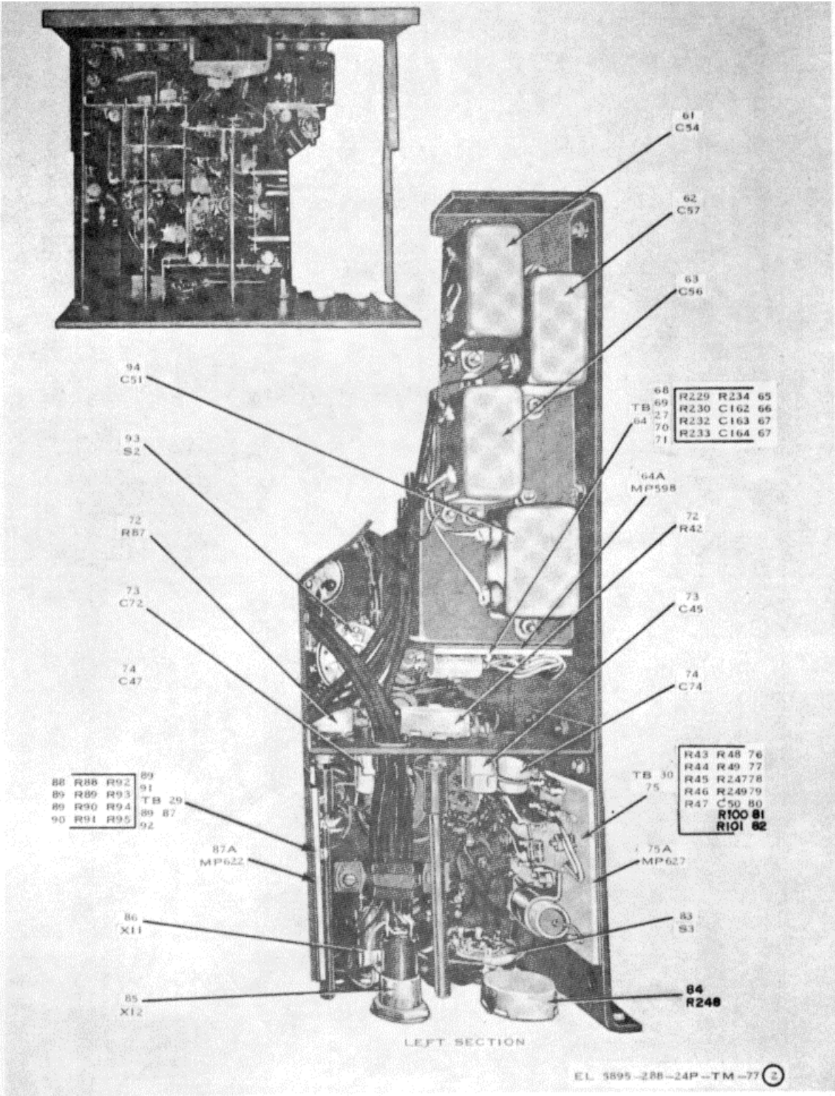
Figure 77. Converter Drawer Assembly, Bottom View (Sheet 2 of 4)
