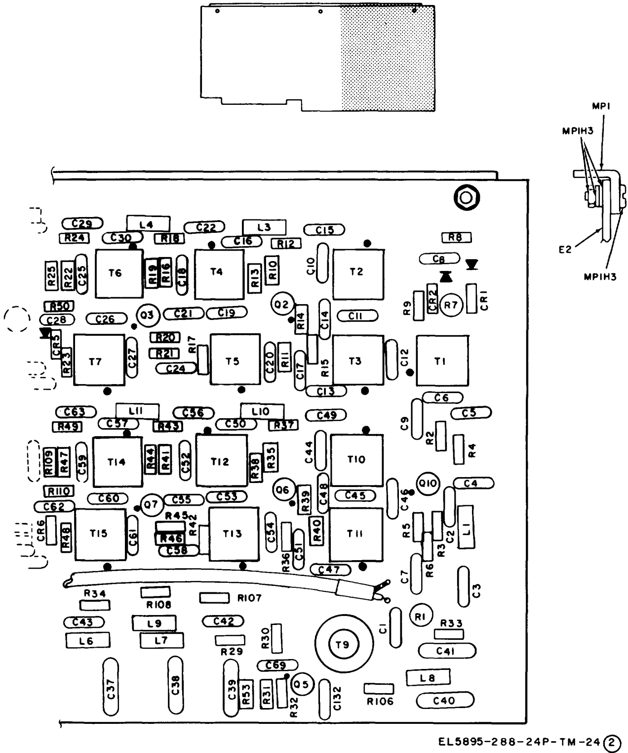
Figure 24. Step Generator A Circuit Card Z110 (Sheet 2 of 2)
