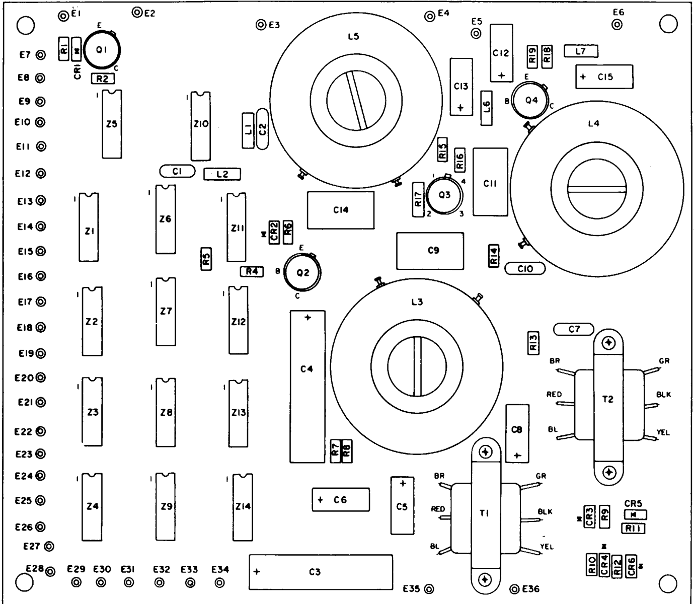
Figure 66. Programmable Divider Circuit Card Z104
