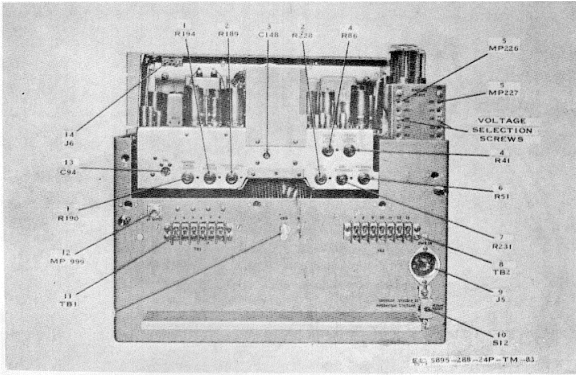
Figure 83. Converter, Rear View, Dust Cover Removed
