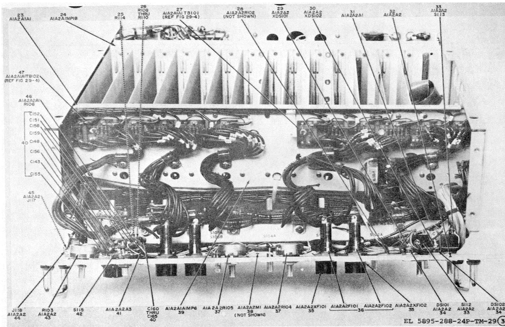
Figure 29. Multimode Exciter Subassembly A1A2 (Sheet 3 of 6)
