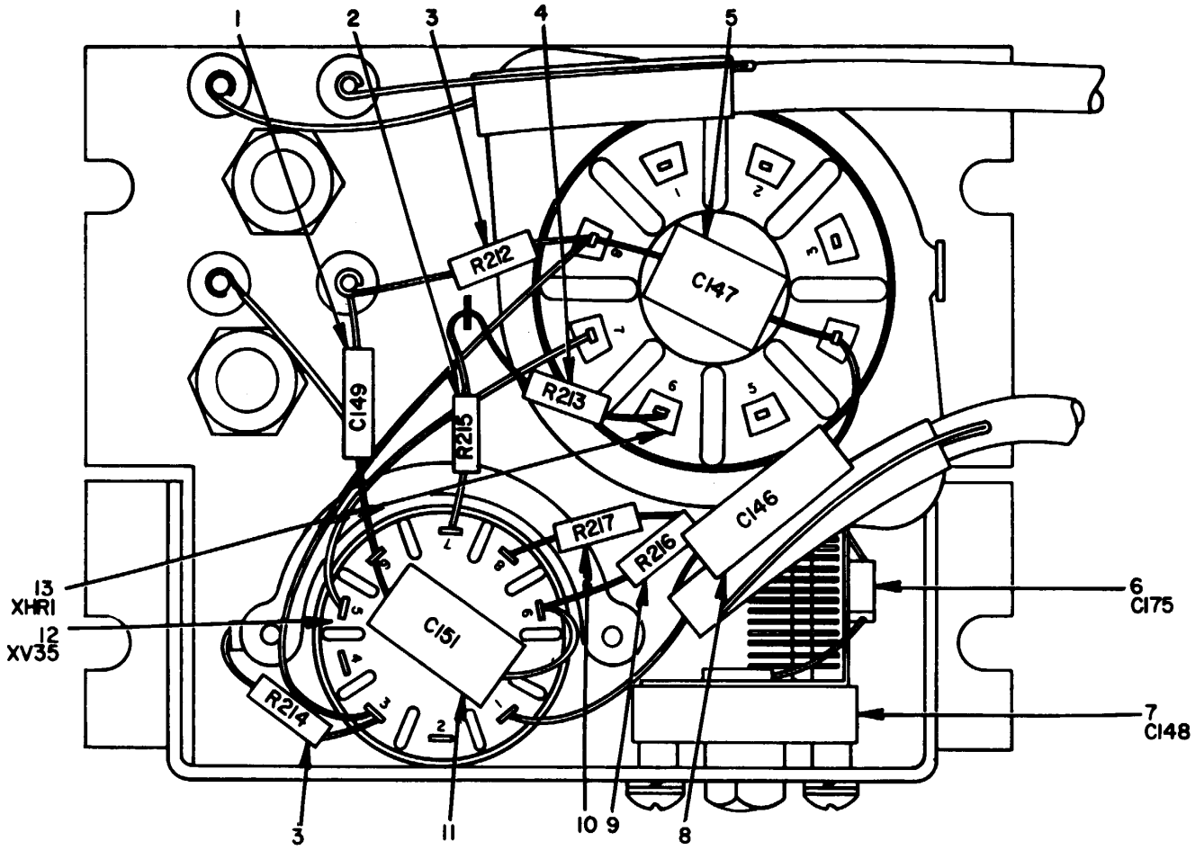
Figure 78. Oscillator Section, Bottom view
