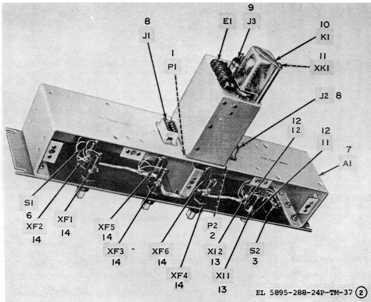
Figure 37. Line Battery Supply No. 1 Panel, NRC Type 227 ( Sheet 2 of 2)
