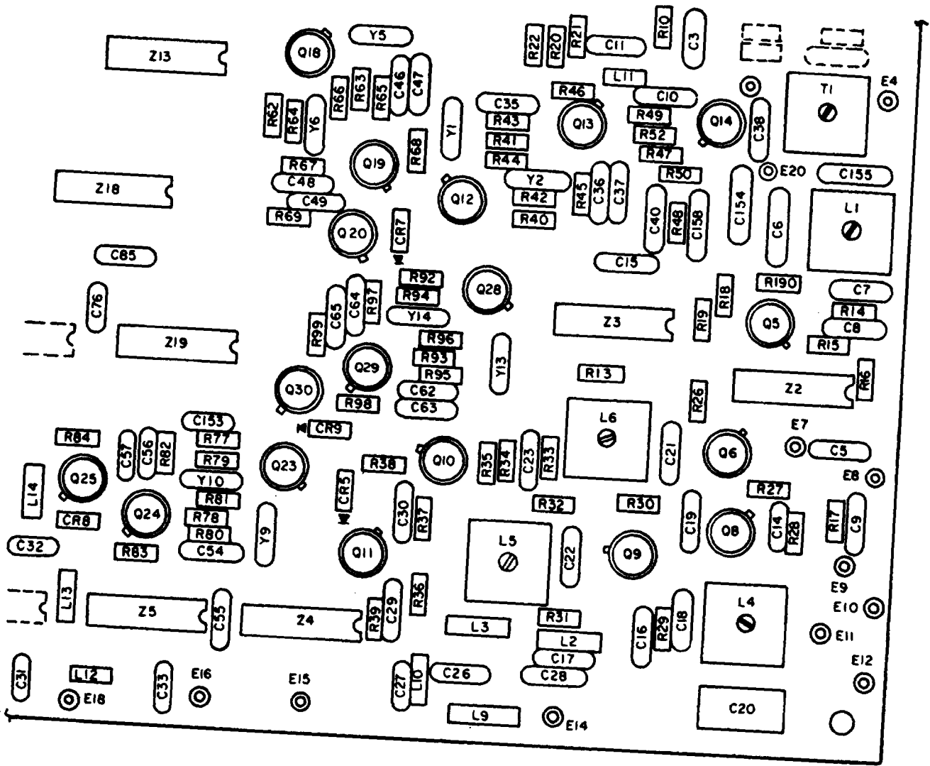
Figure 73. Spectrum Generator Circuit Card Z102 (Sheet 4 of 4)
