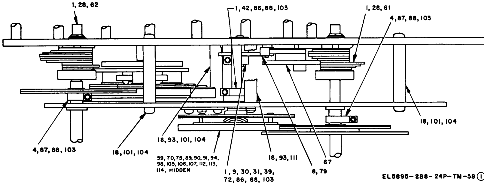
Figure 58. Gear Train Assembly A1A9 (Sheet 1 of 6)
