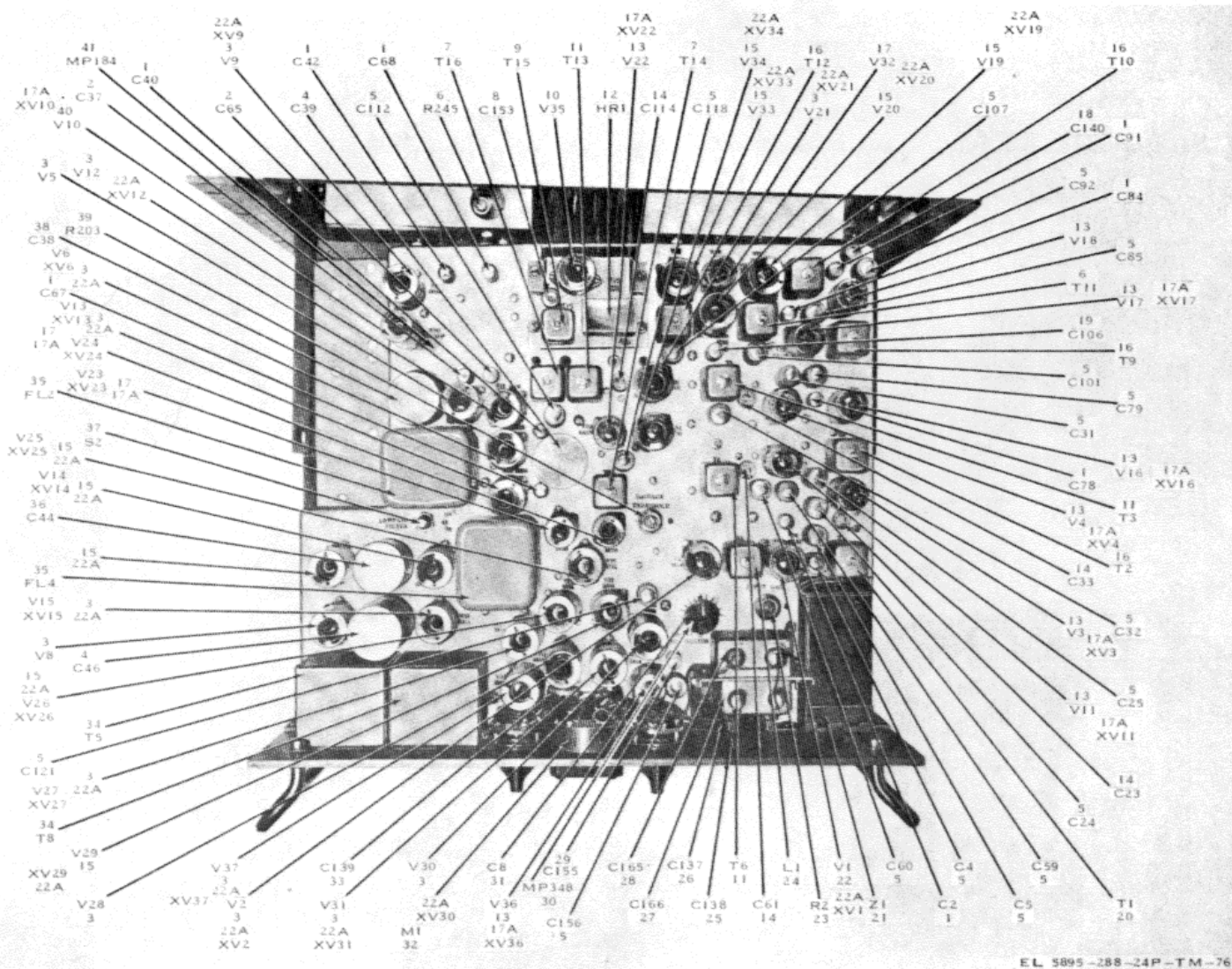
Figure 76. Converter Drawer Assembly, Top View
