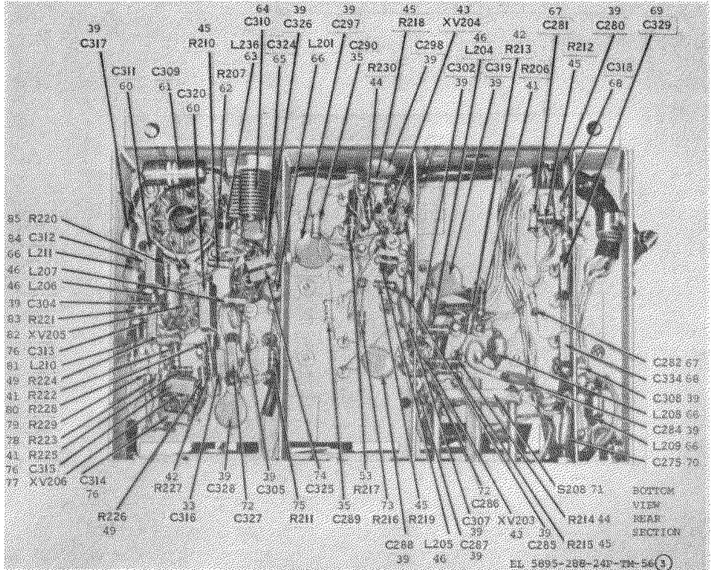
Figure 56. Radio Frequency Amplifier A1A7 (Sheet 3 of 3)
