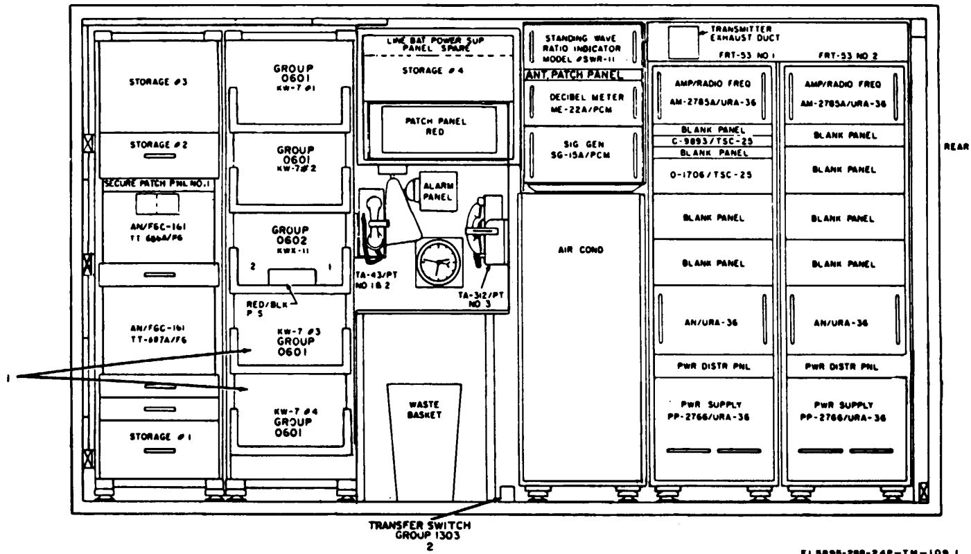
Figure 109.1. Miscellaneous Group
