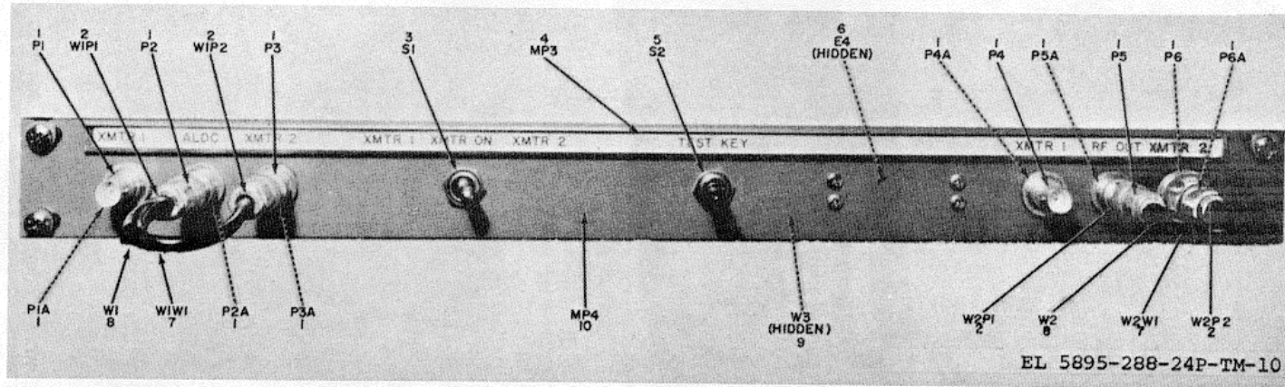
Figure 10. Control Transmitter C-9893/TSC-25
