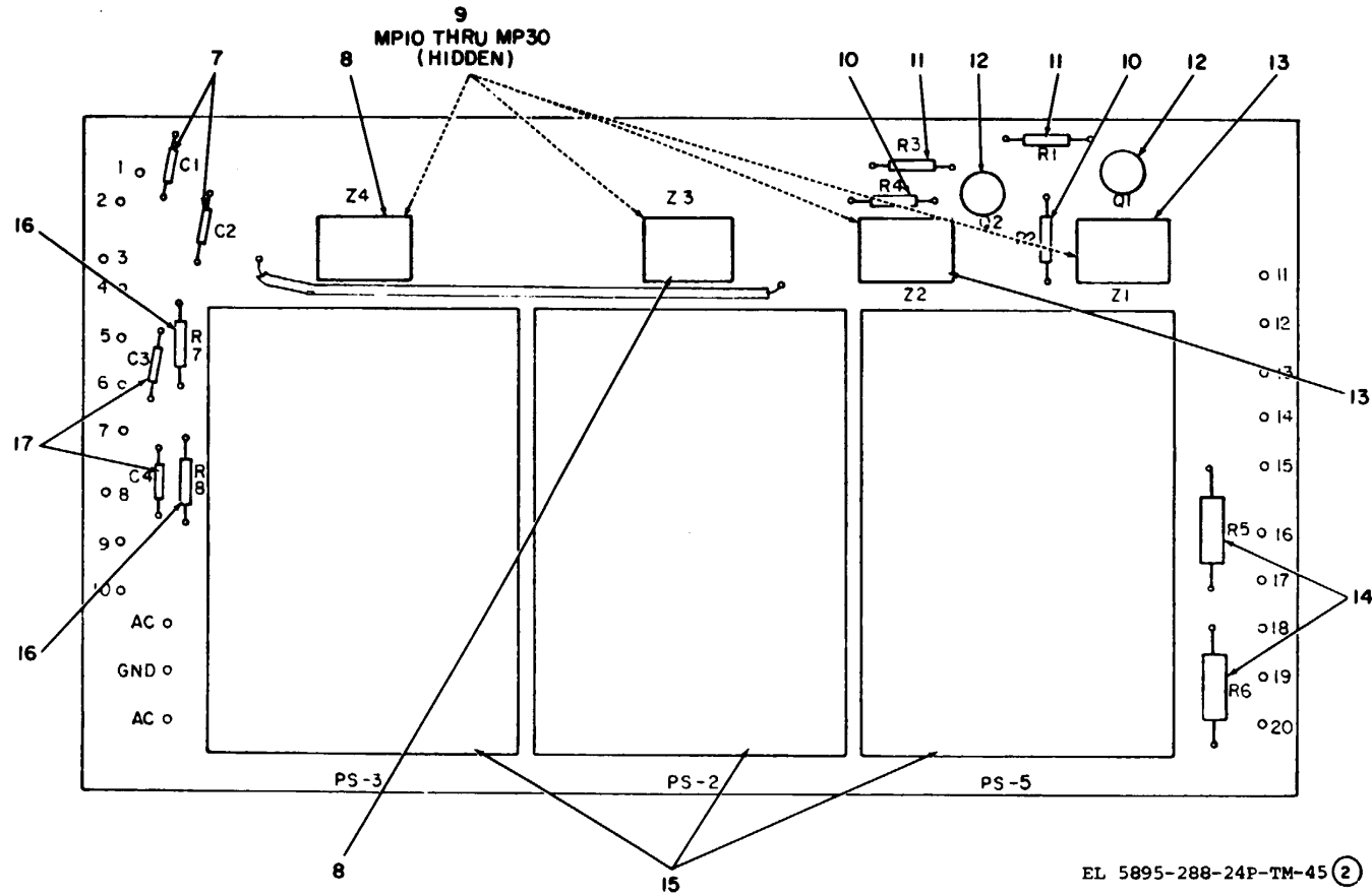
Figure 45. Low Level Interface No. 1 Box (Sheet 2 of 2)
