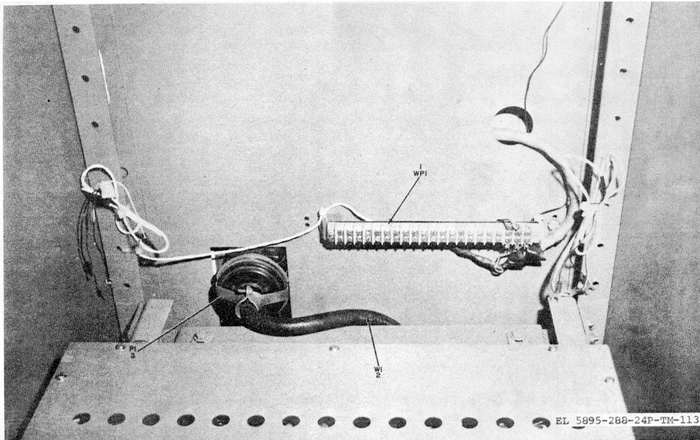
Figure 113. Electrical Power Cable, Rack 408
