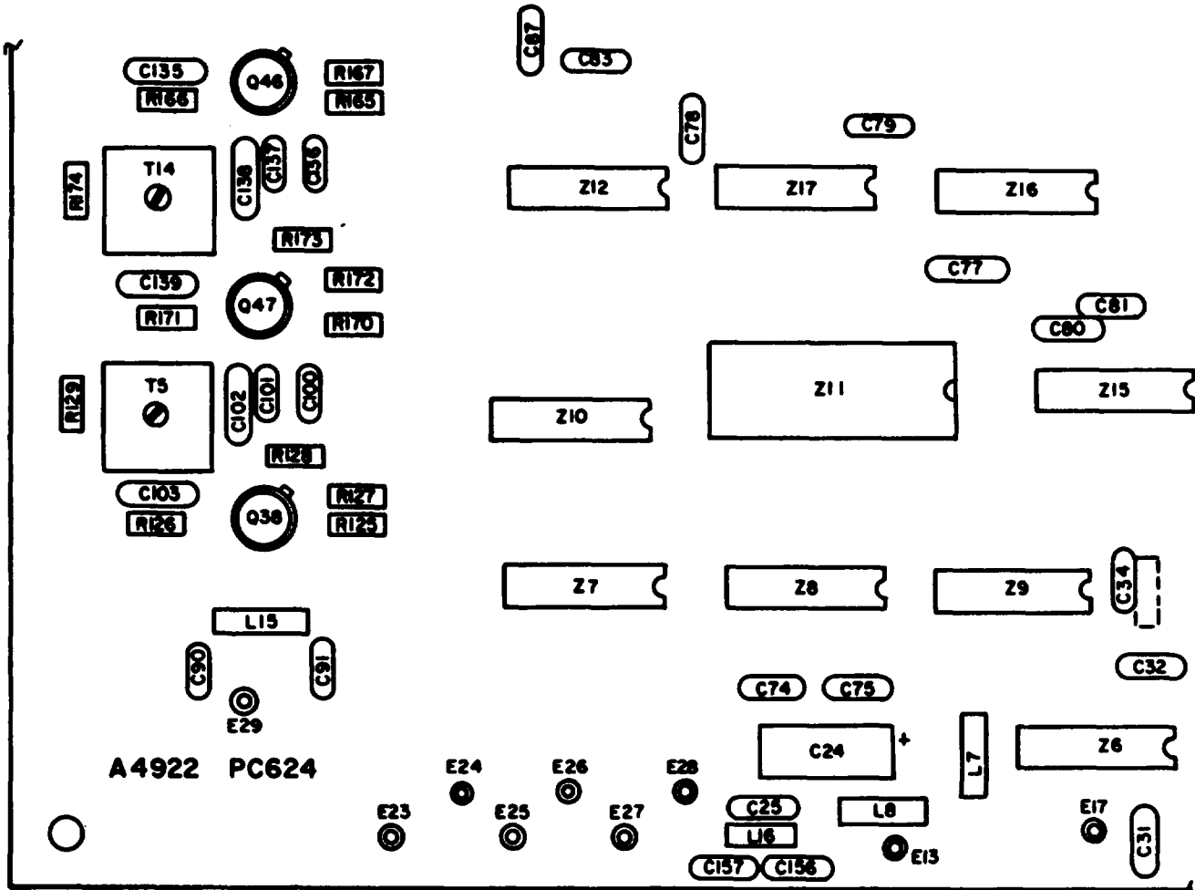
Figure 73. Spectrum Generator Circuit Card Z102 (Sheet 3 of 4)
