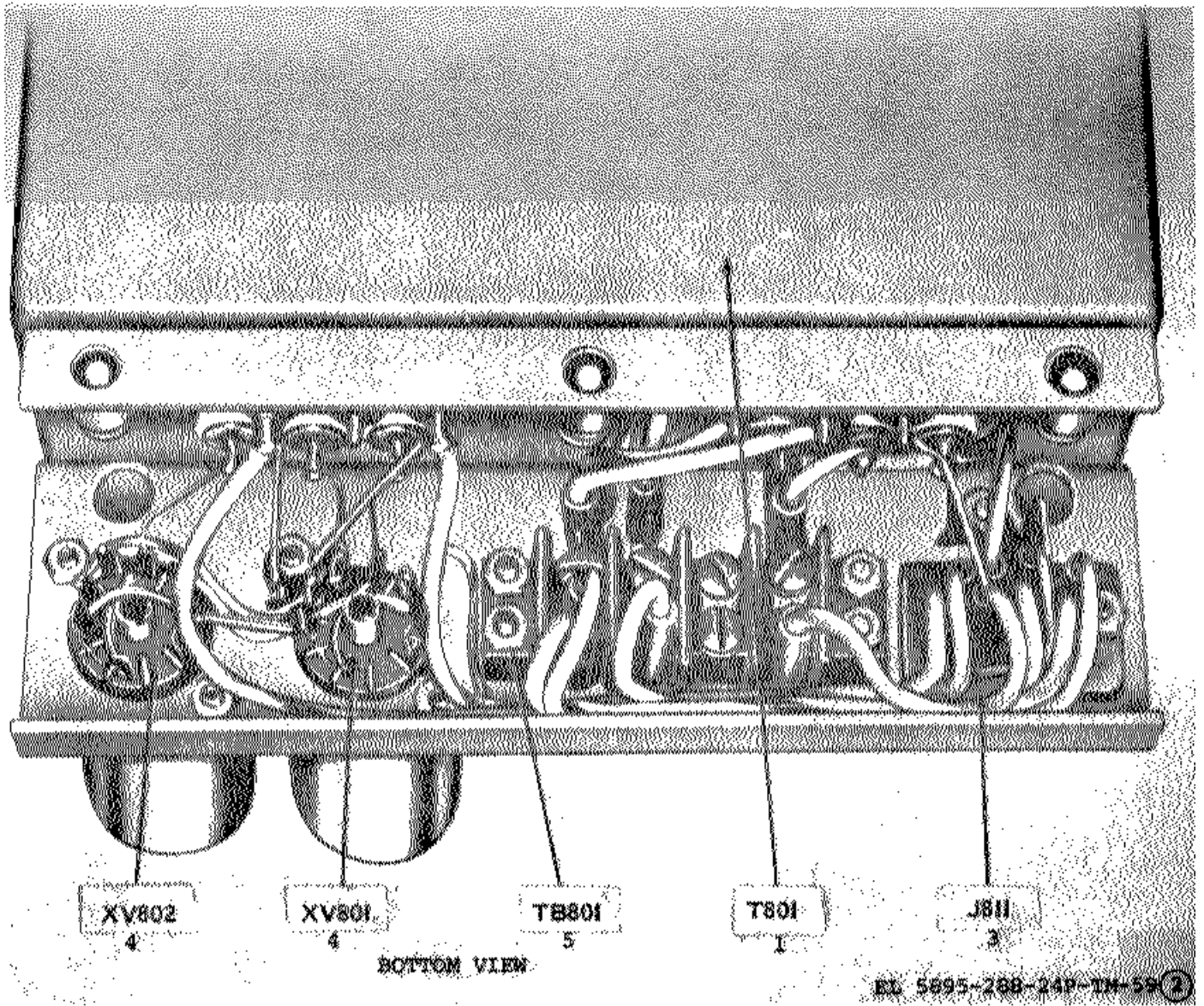
Figure 59. Power Supply Subchassis A1A5 (Sheet 1 of 2)
