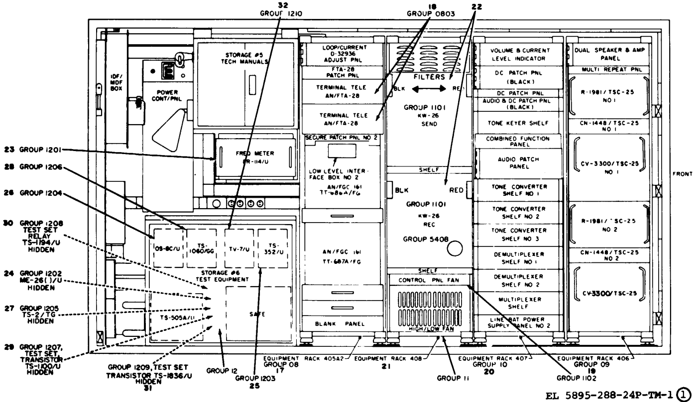
Figure 1. Communications Central AN/TSC-25 (Sheet 1 of 2)
