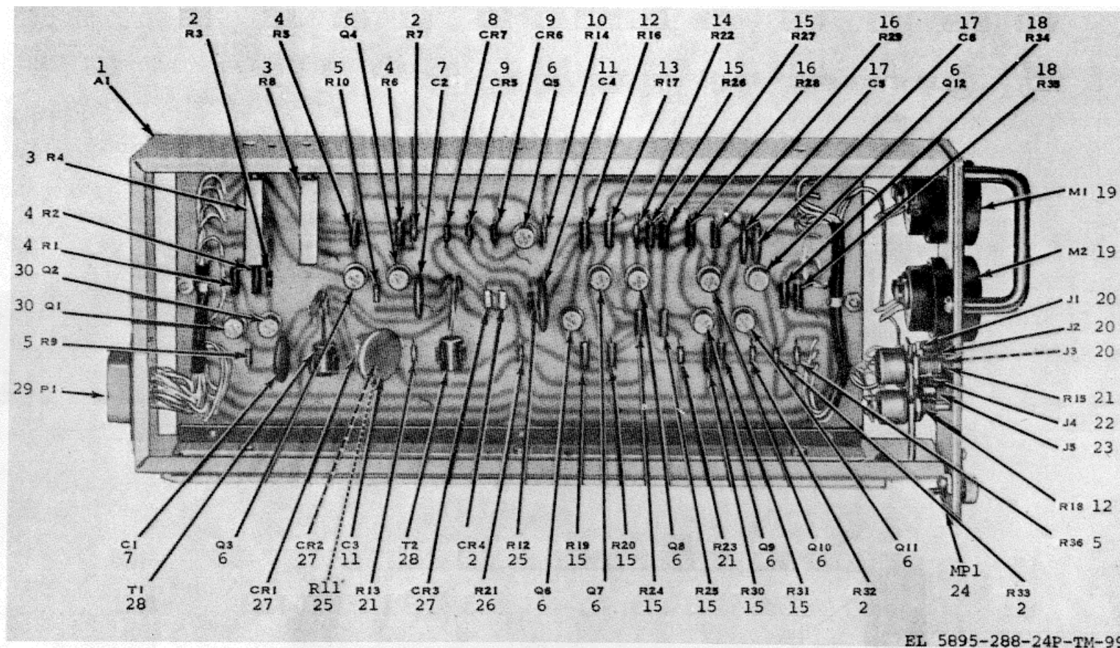
Figure 99. Diversity Combiner, Type 234, Model 2
