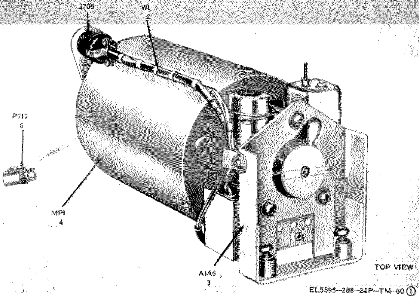
Figure 60. Radio Frequency Oscillator A1A6 (Sheet 1 of 2)
