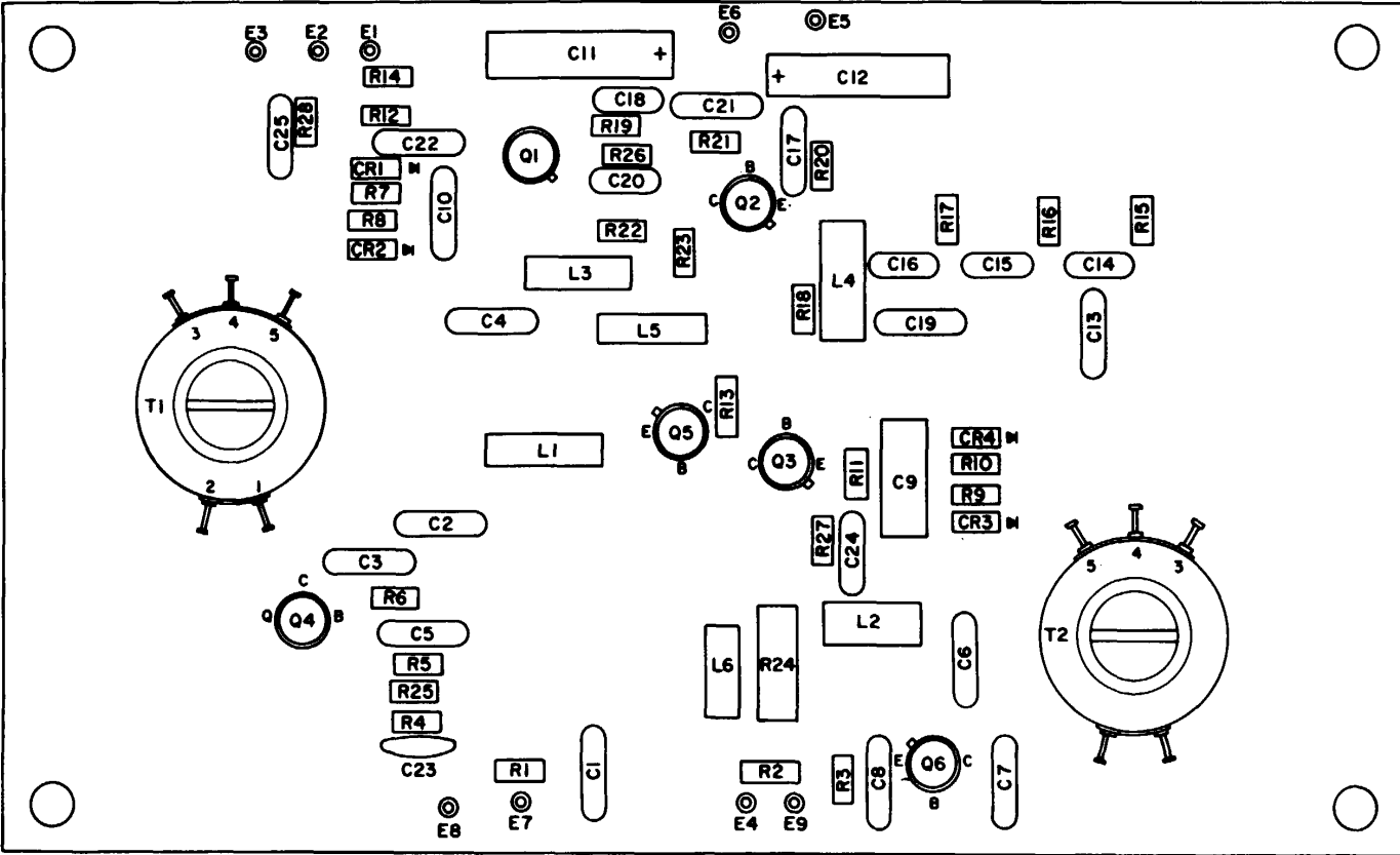
Figure 70. Phase Detector Circuit Card Z109
