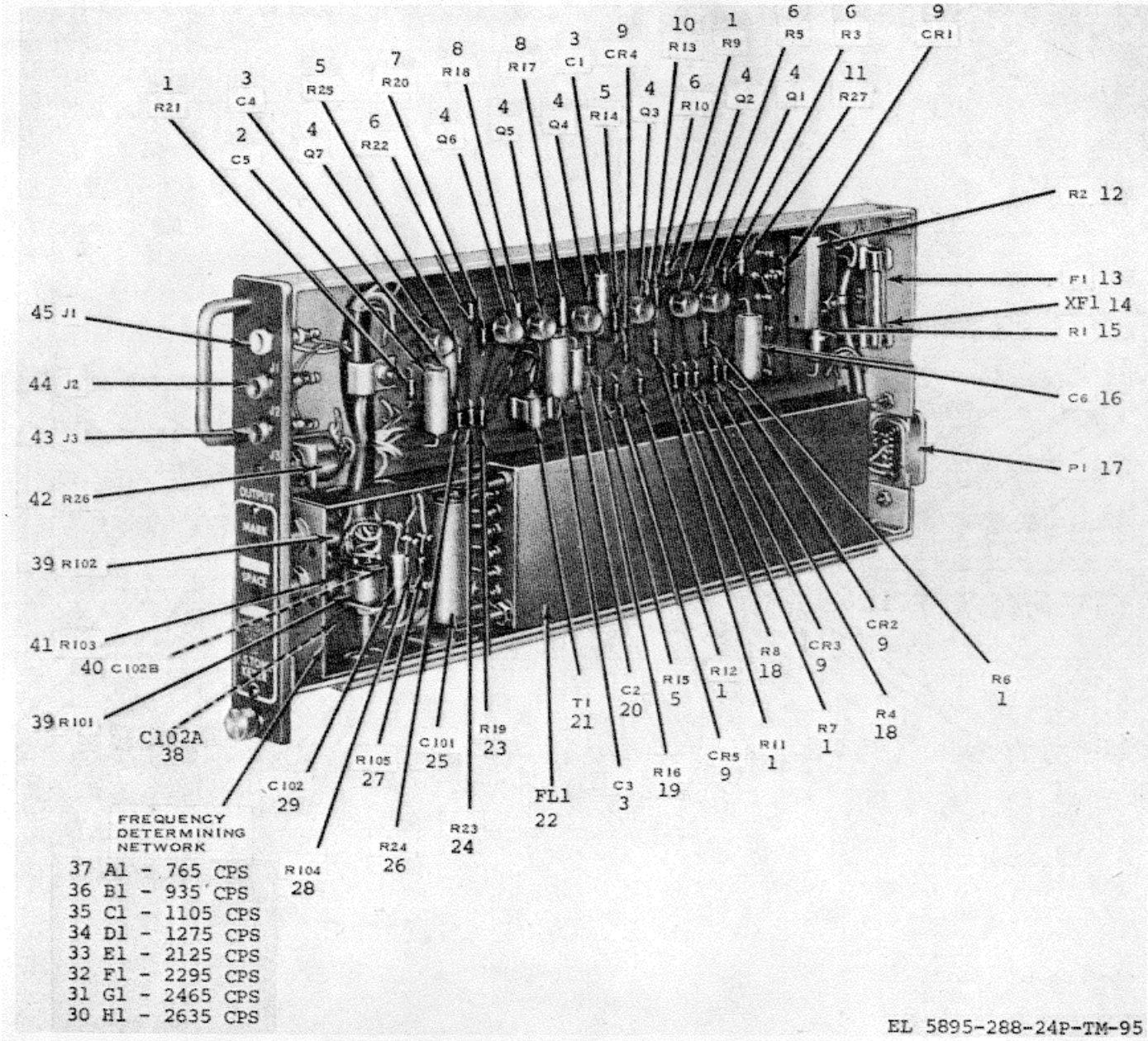
Figure 95. Frequency Shift Tone Keyer Type 211, Model 2
