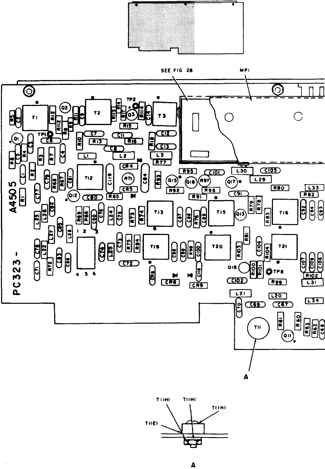
Figure 27. Translater Circuit Card Z112 (Sheet 1 of 2)
