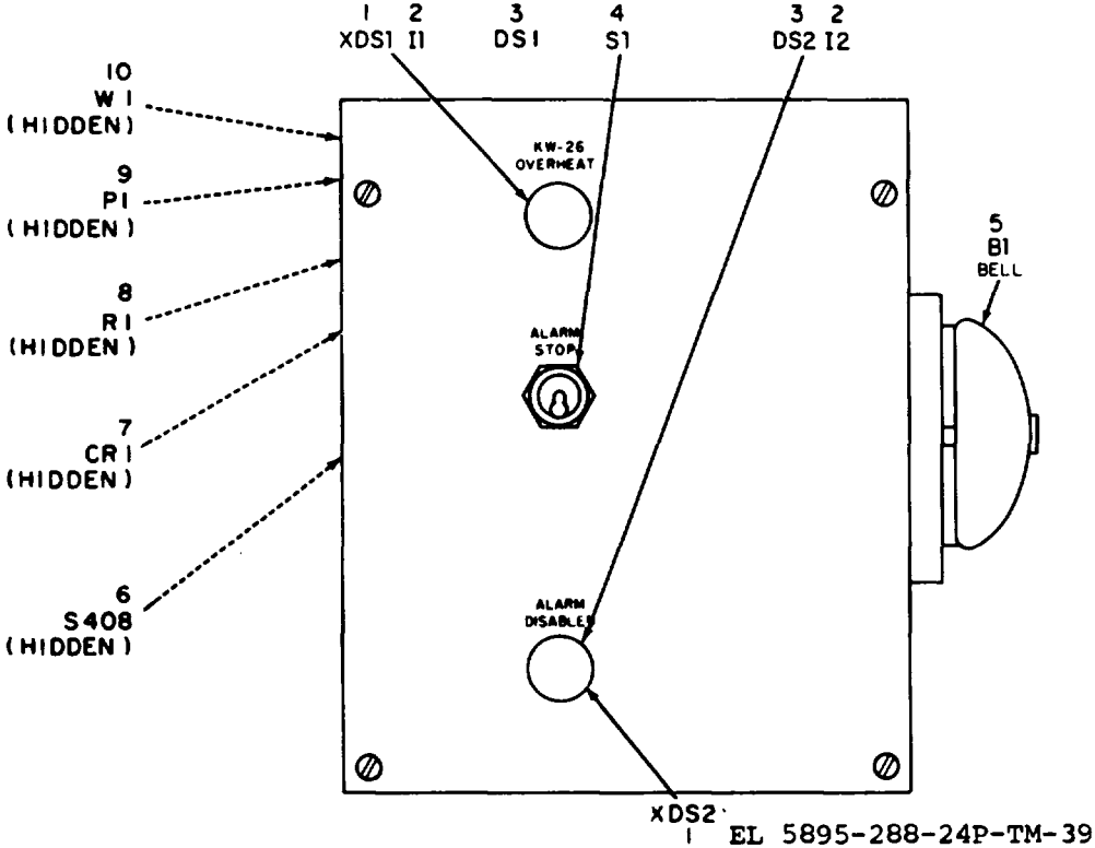
Figure 39. Alarm Unit
