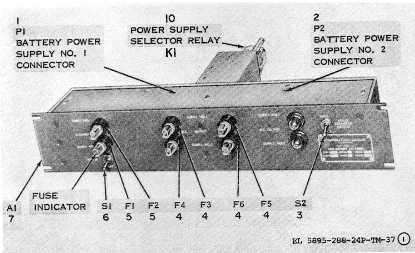
Figure 37. Line Battery Supply No. 1 Panel, NRC Type 227 (Sheet 1 of 2)
