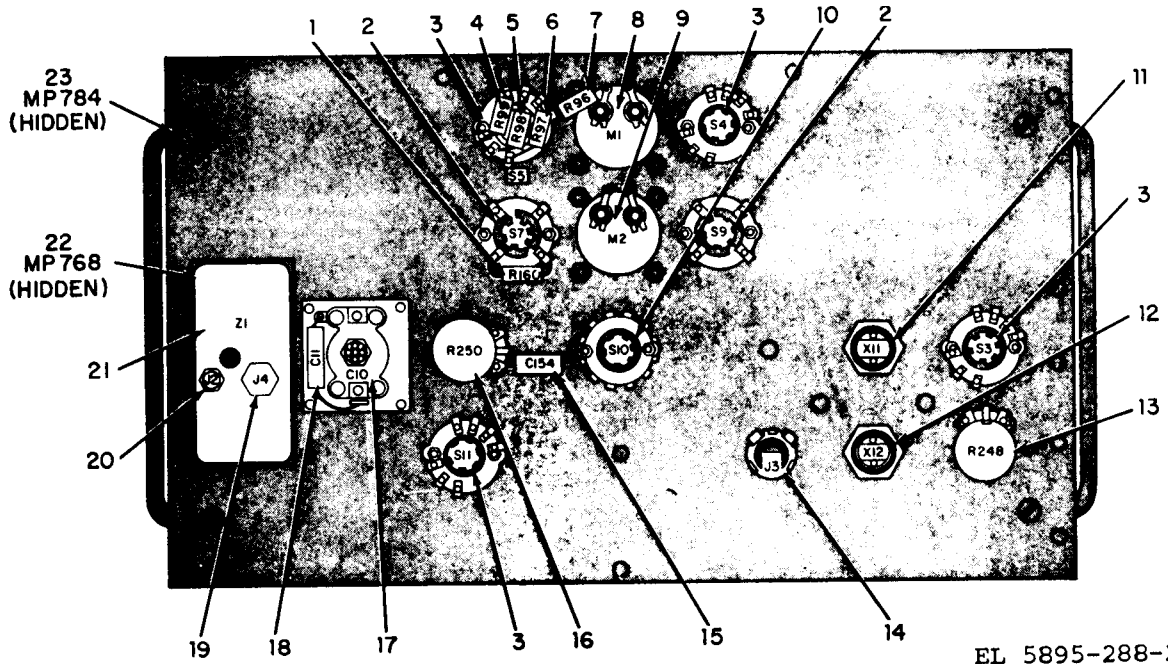
Figure 79. Control Panel, Rear View
