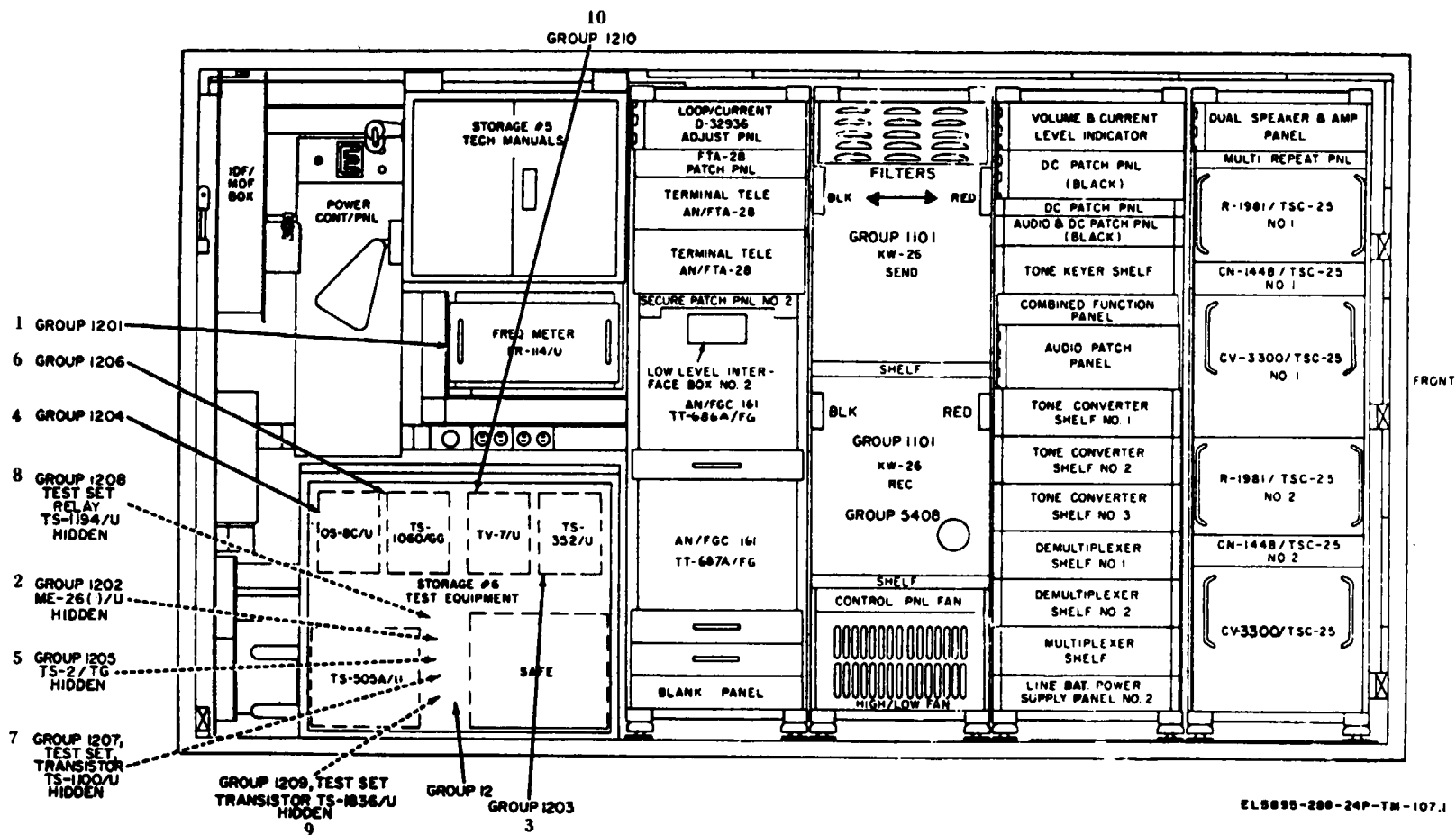
Figure 107.1. Test Equipment
