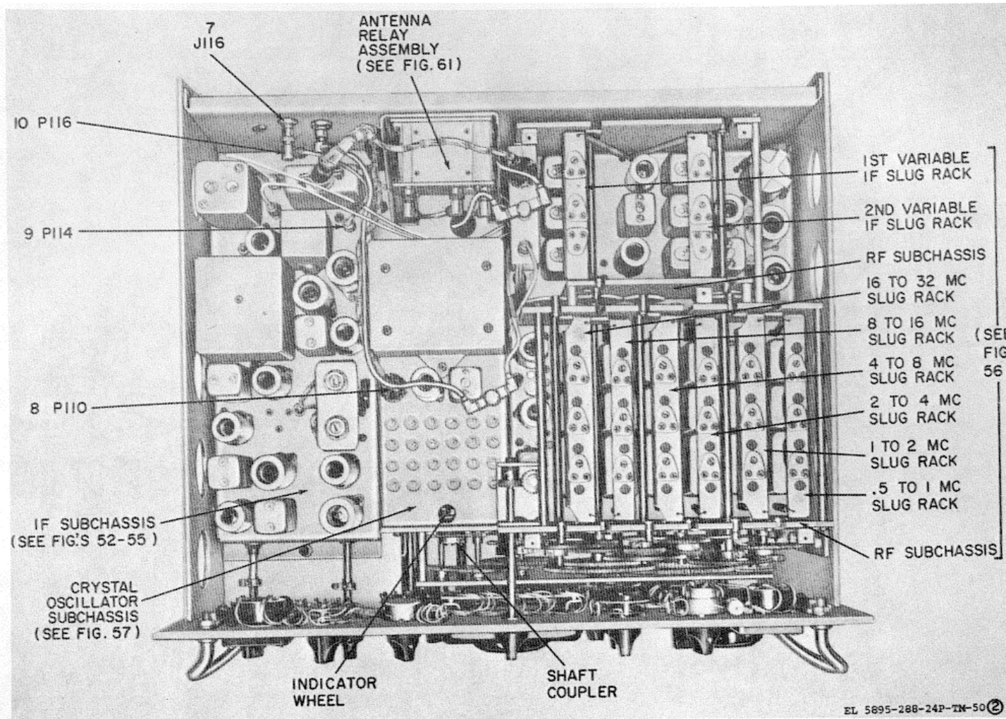
Figure 50. Radio Receiver R-1981/TSC-25 (Sheet 2 of 3)
