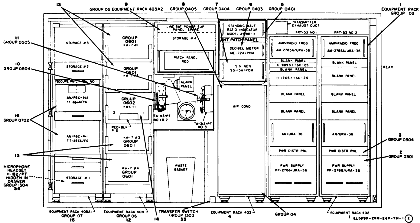
Figure 1. Communications Central AN/TSC-25 (Sheet 2 of 2)
