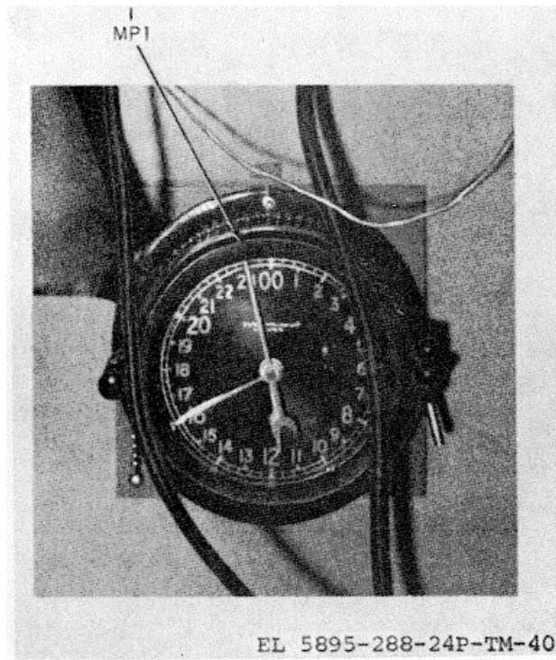
Figure 40. Clock
