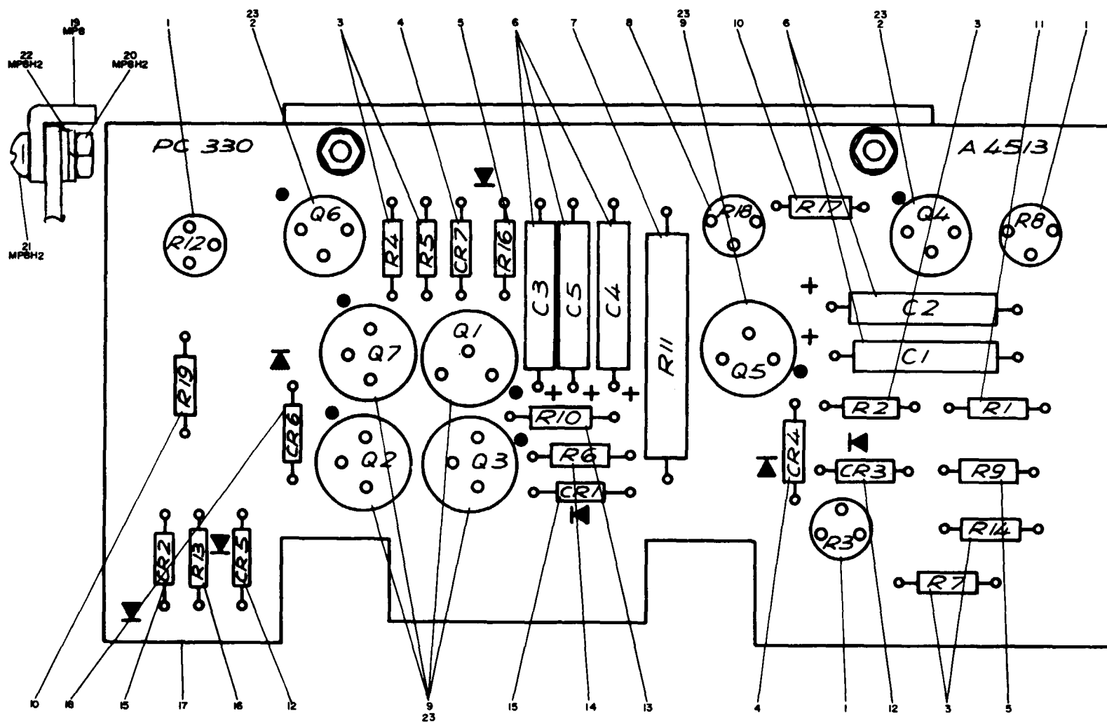
Figure 32. Circuit Card B Z303
