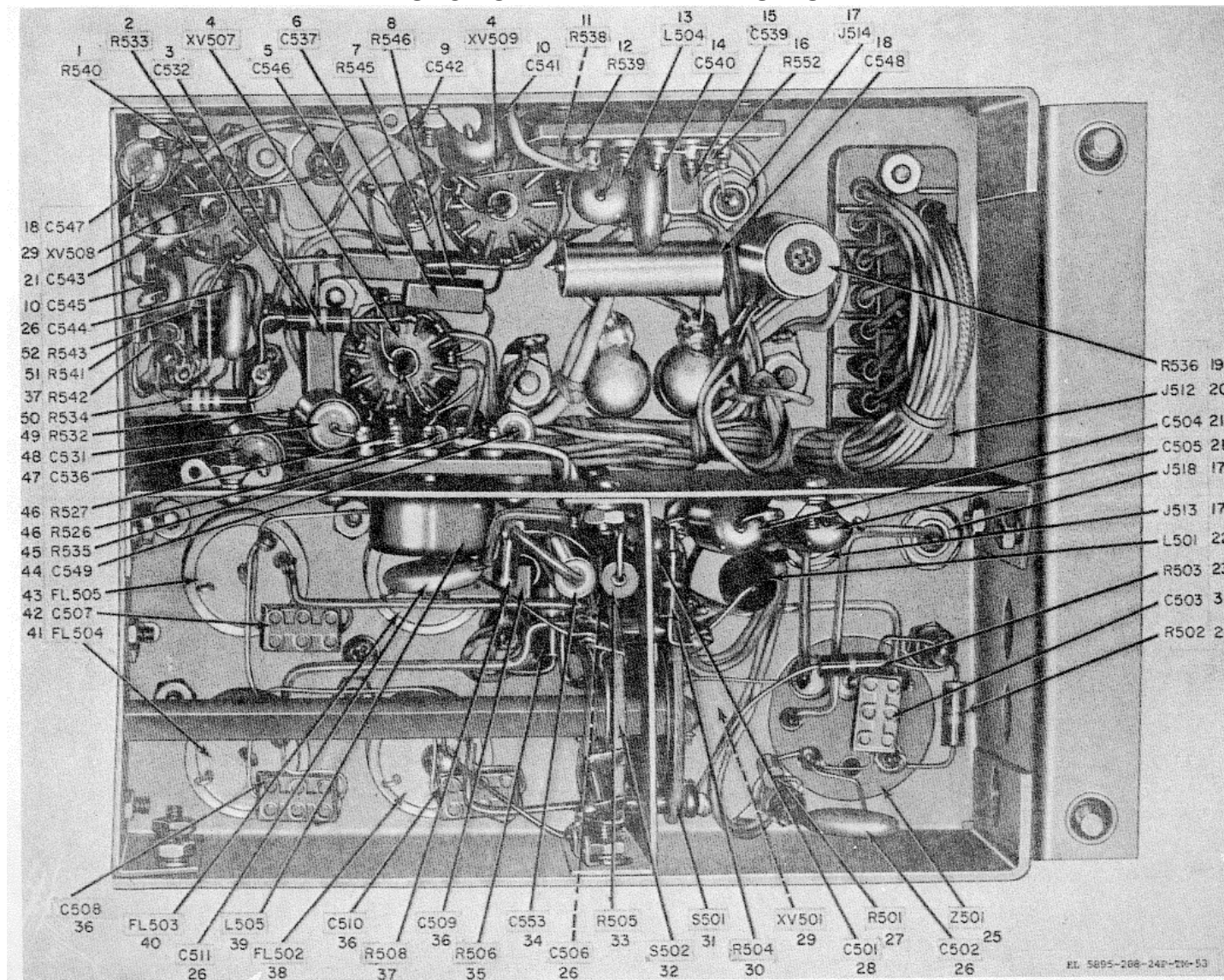
Figure 53. Unmodified IF Subchassis, Bottom View, Rear Section
