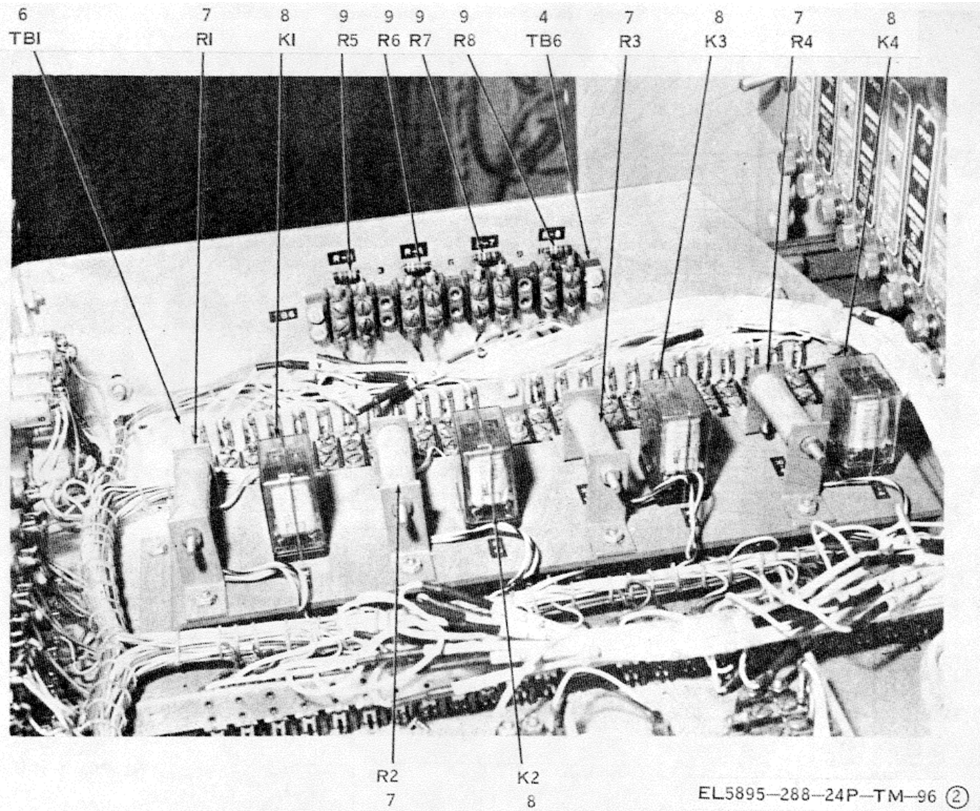
Figure 96. Combined Function Panel (Sheet 2 of 3)
