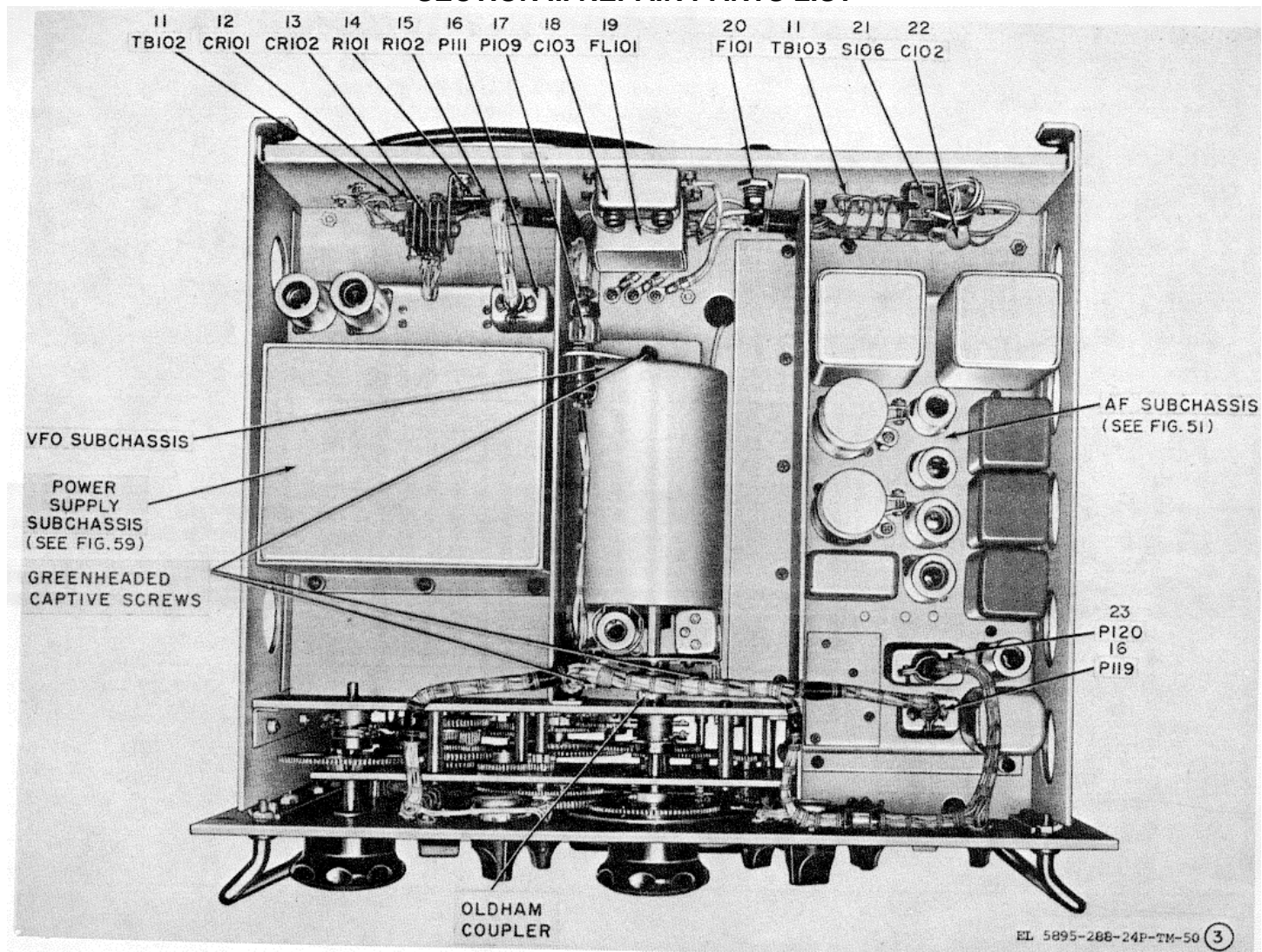
Figure 50. Radio Receiver R-1981/TSC-25 (Sheet 3 of 3)
