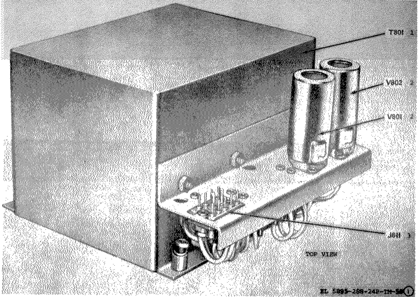
Figure 59. Power Supply Subchassis A1A5 (Sheet 1 of 2)
