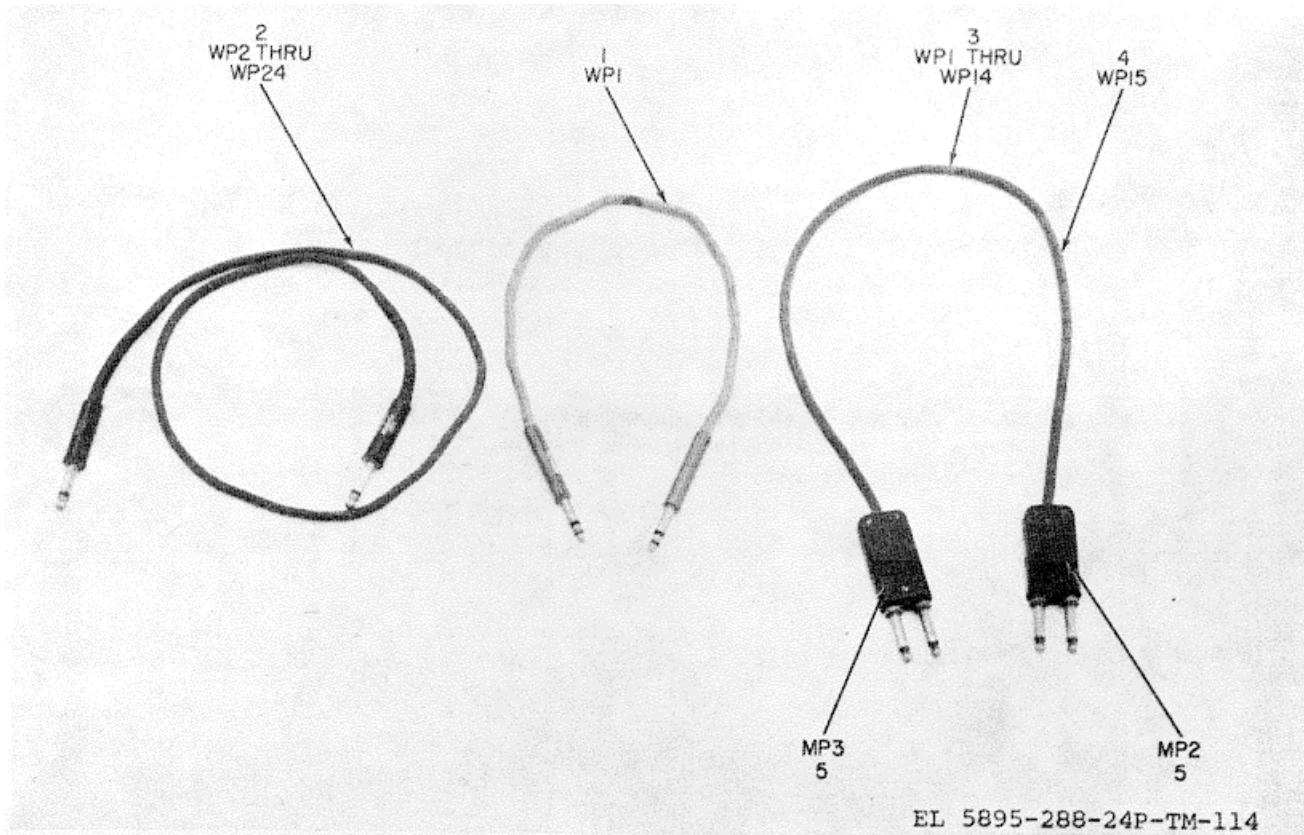
Figure 114. Cord Assemblies
