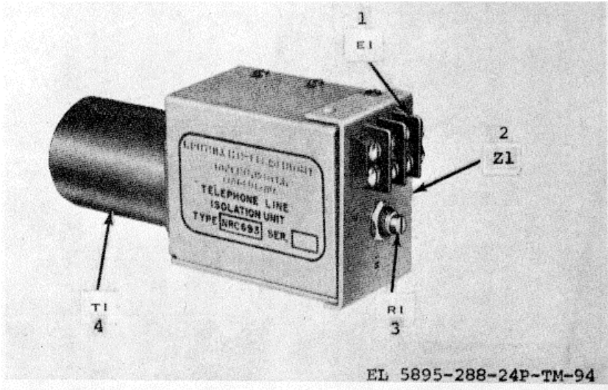
Figure 94. Telephone Line Isolation Unit Z1
