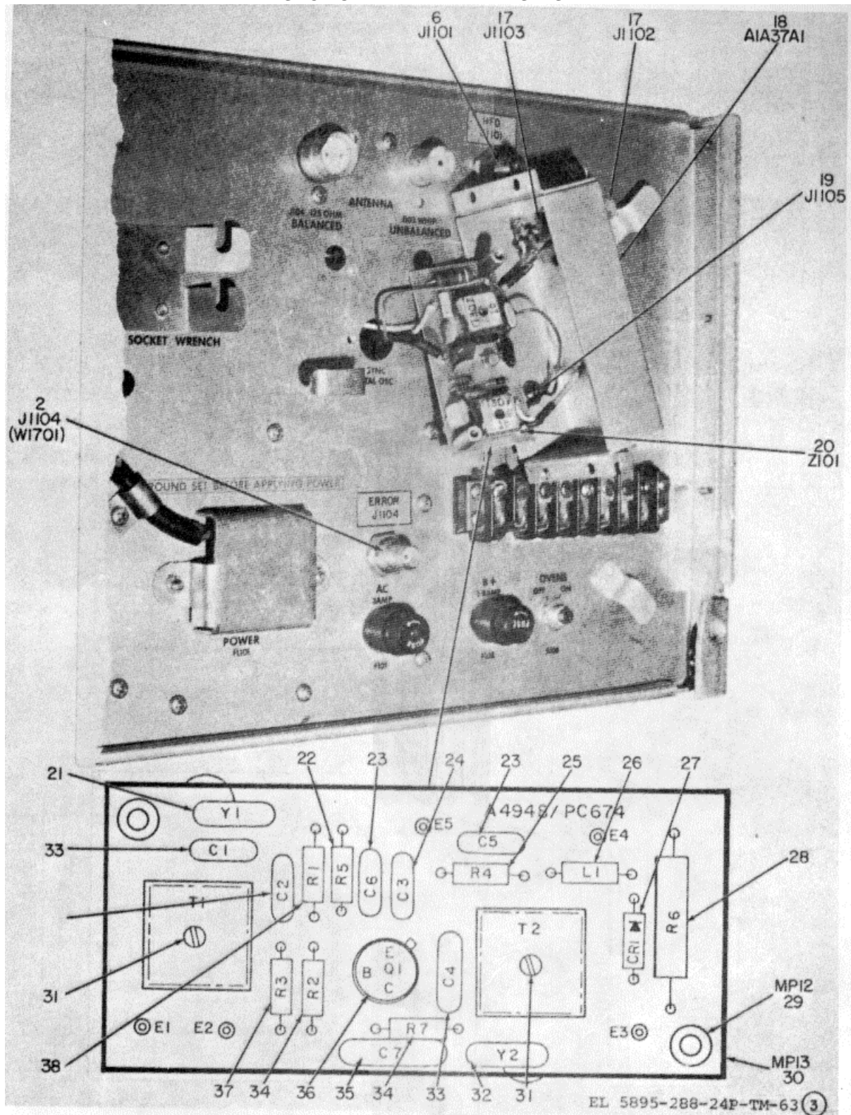
Figure 63. Radio Receiver Modification (Sheet 3 of 3)
