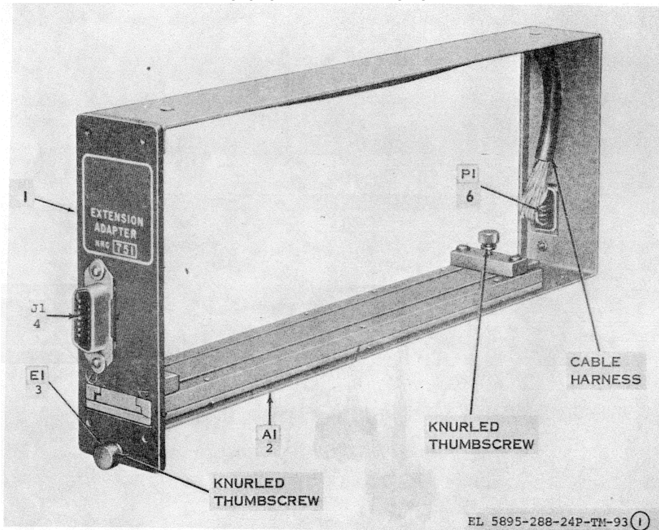
Figure 93. Extension Adapter AI, Models 750 and 751 (Sheet 1 of 2)
