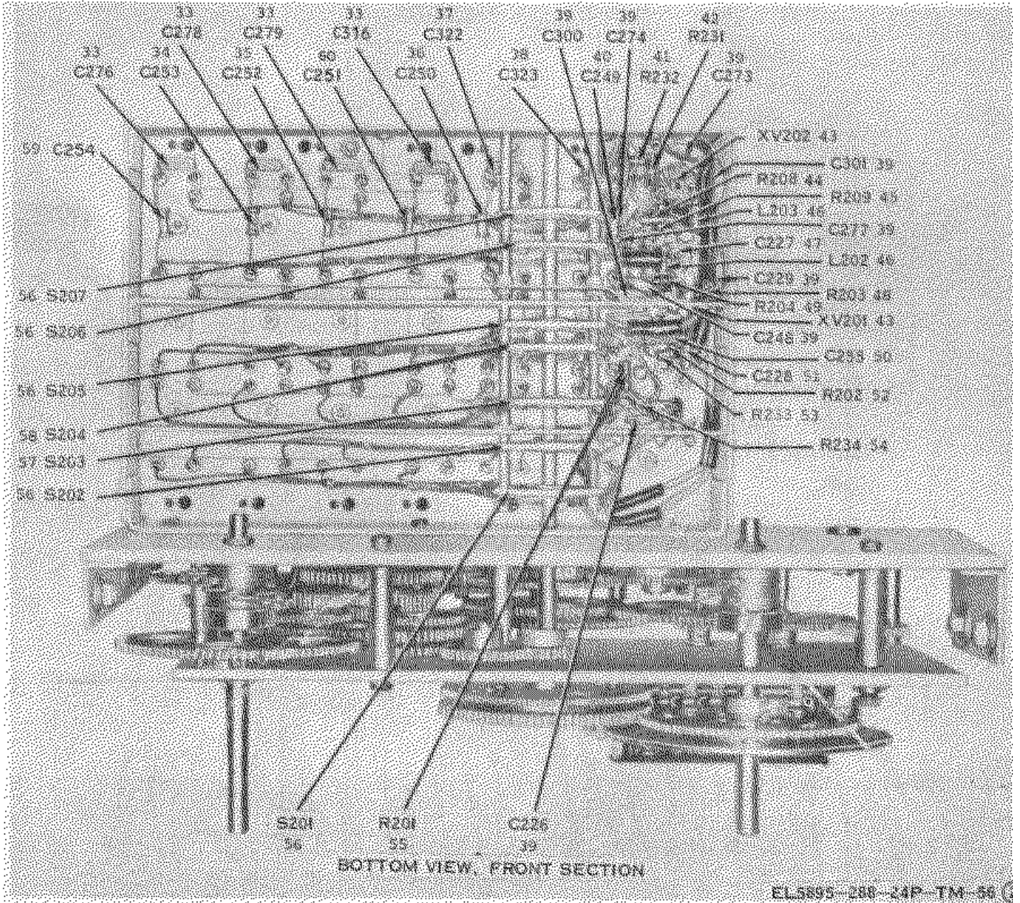
Figure 56. Radio Frequency Amplifier A1A7 (Sheet 2 of 3)
