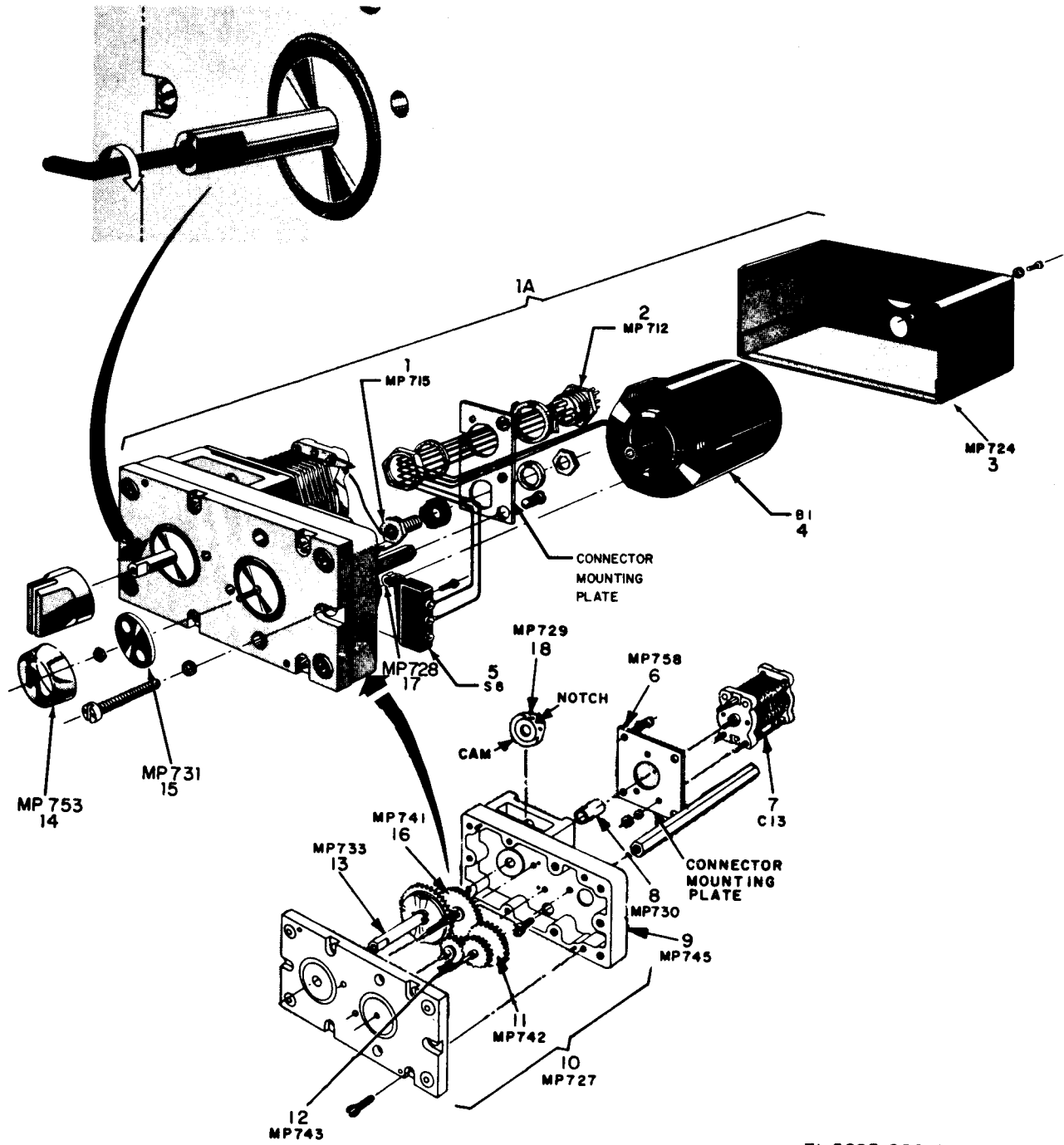
Figure 85. AFC Unit, Exploded View
