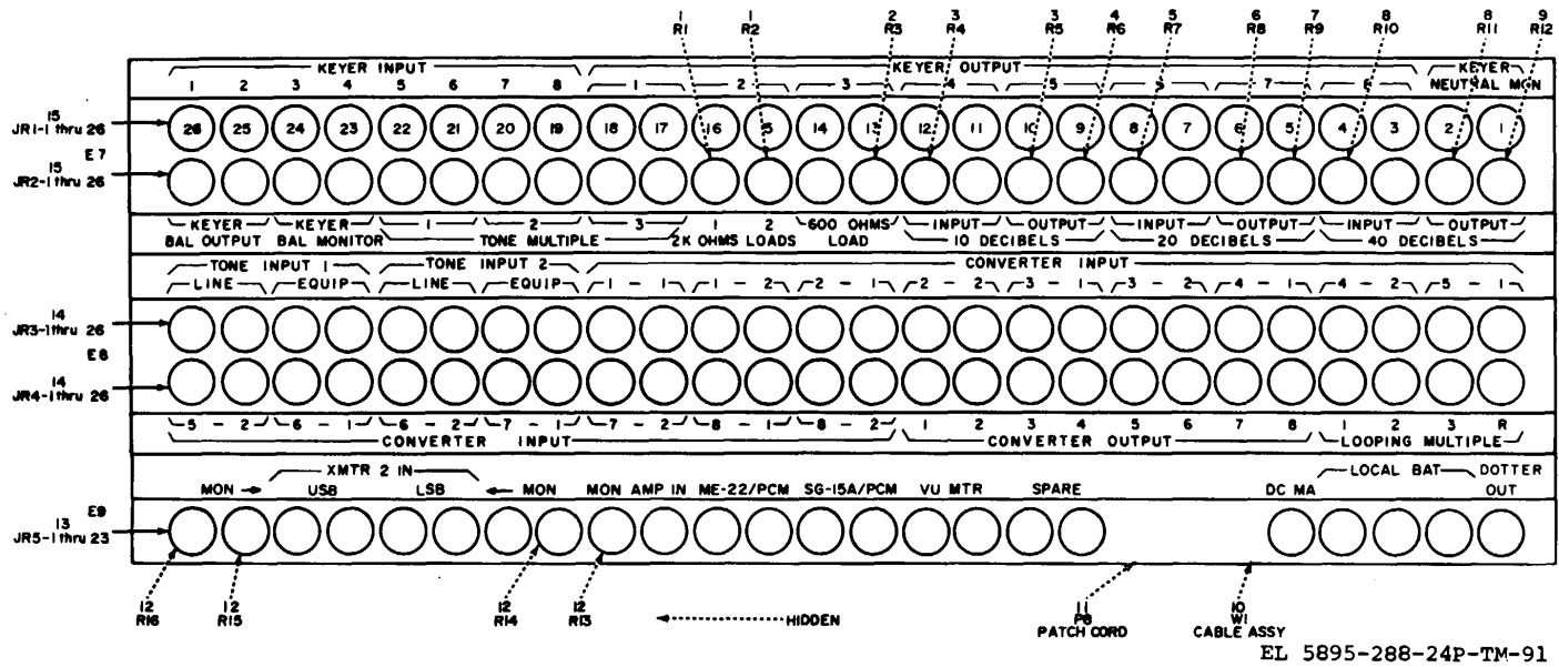
Figure 91. Audio-DC Patch Panel
