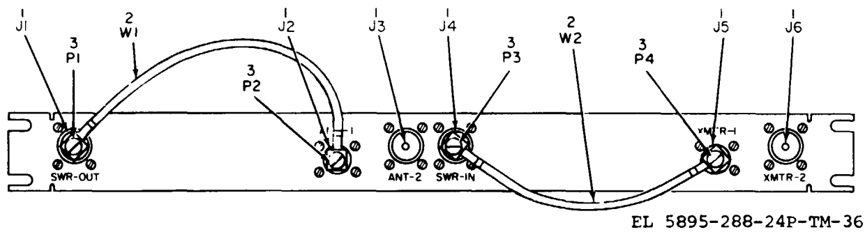
Figure 36. Antenna Patch Panel
