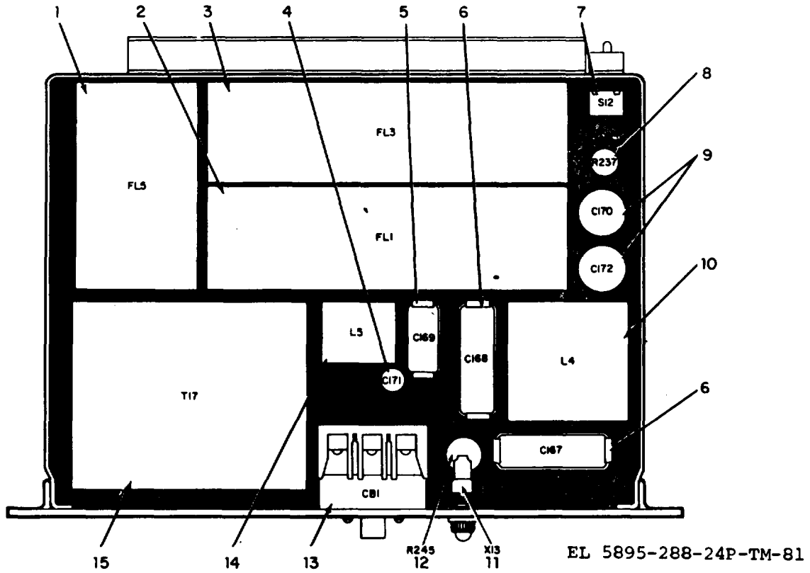
Figure 81. Converter Base Assembly, Bottom View
