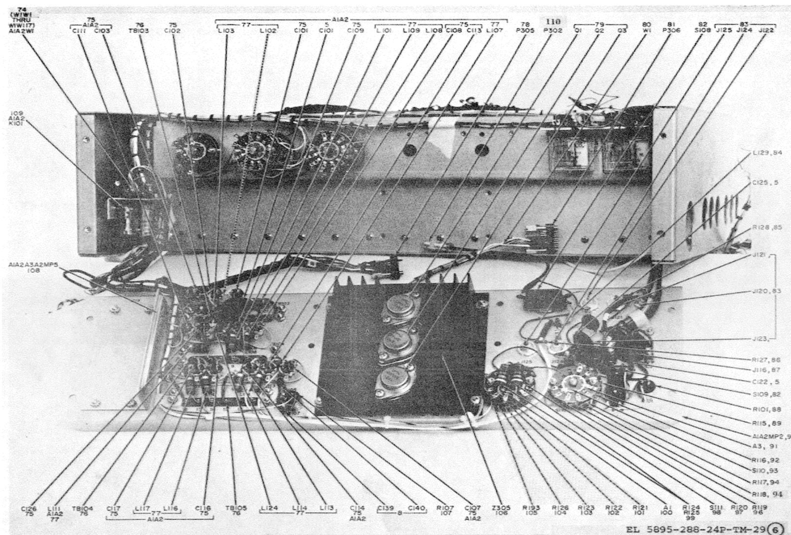
Figure 29. Multimode Exciter Subassembly A1IA2 (Sheet 6 of 6)
