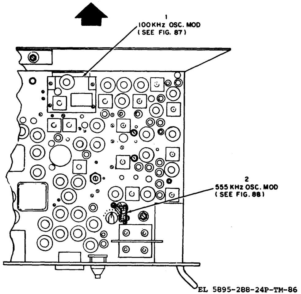
Figure 86. Converter Top and Rear View, Modification
