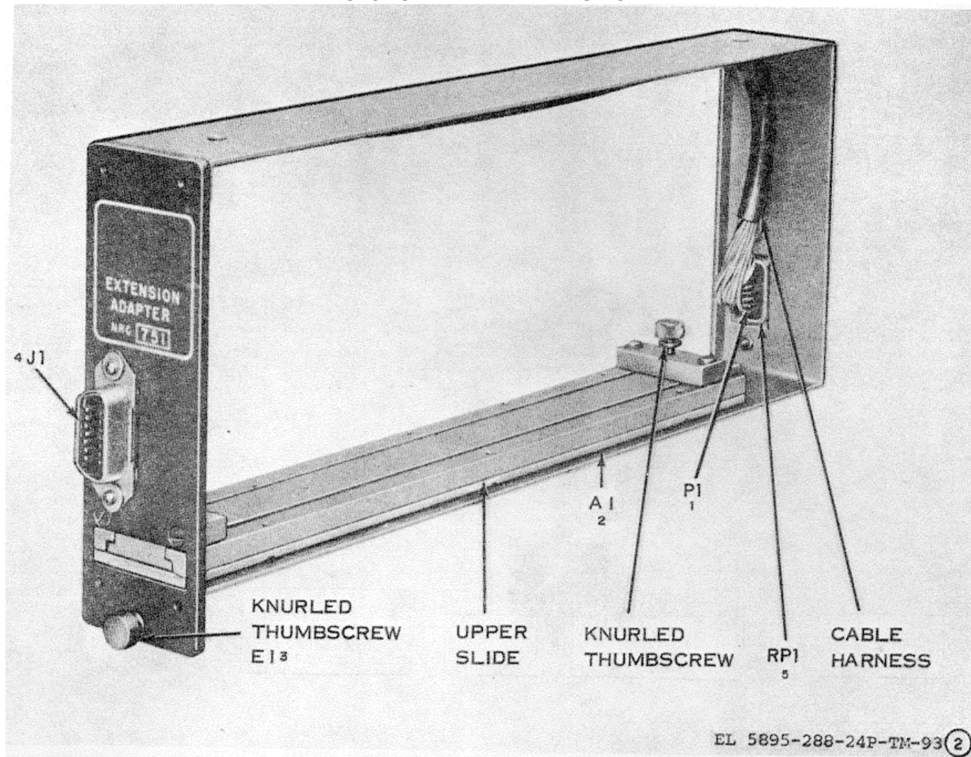
Figure 93. Extension Adapter A1, Models 750 and 751 (Sheet 2 of 2)
