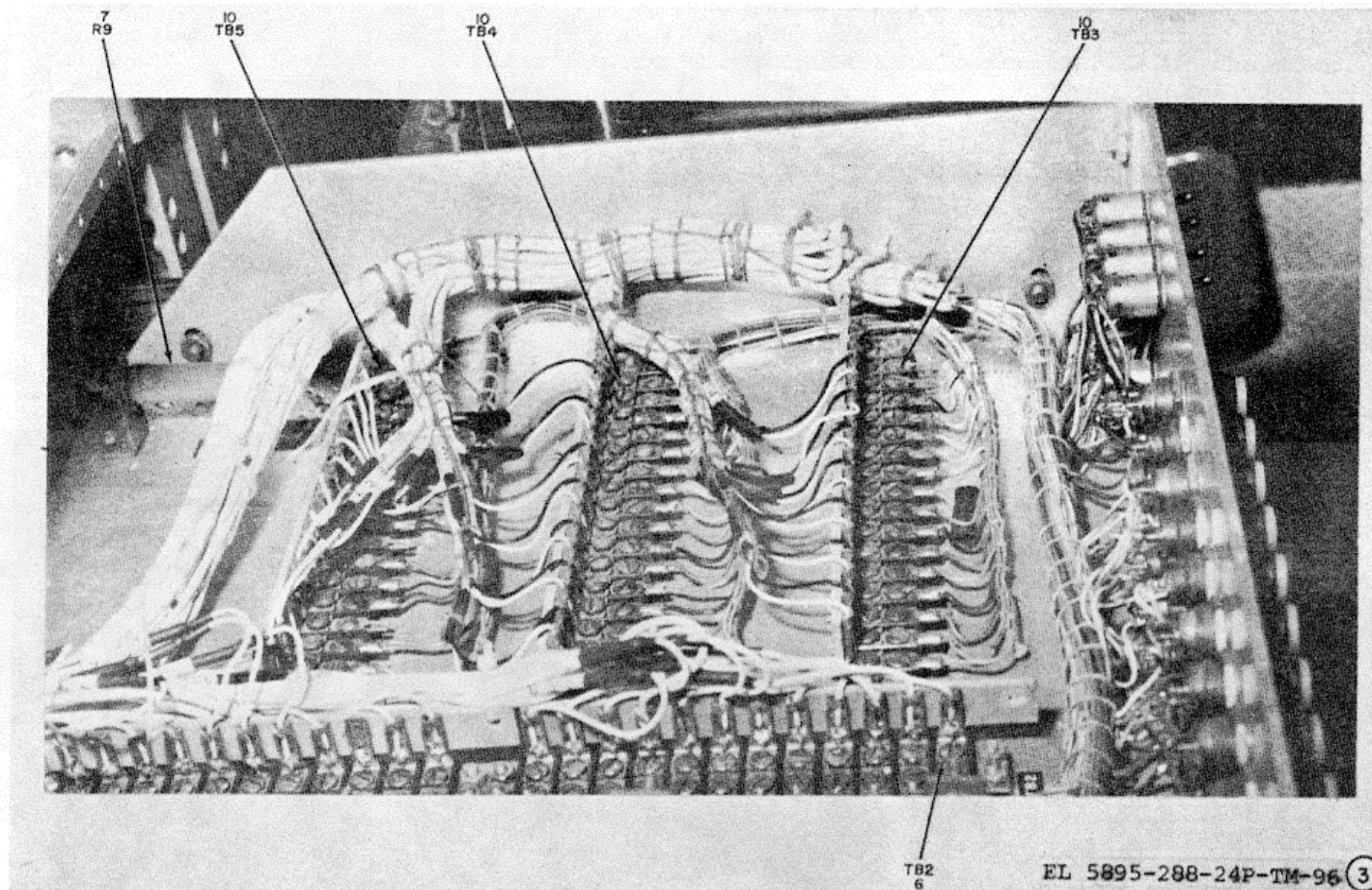
Figure 96. Combined Function Panel (Sheet 3 of 3)
