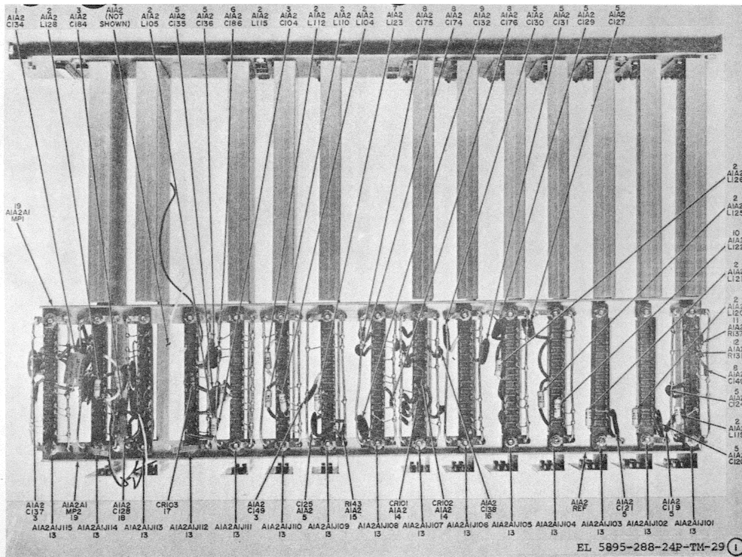
Figure 29. Multimode Exciter Subassembly A1A2 (sheet 1 of 6)
