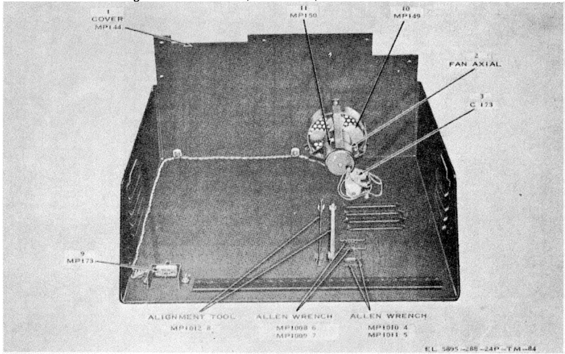
Figure 84. Interior of Converter Dust Cover
