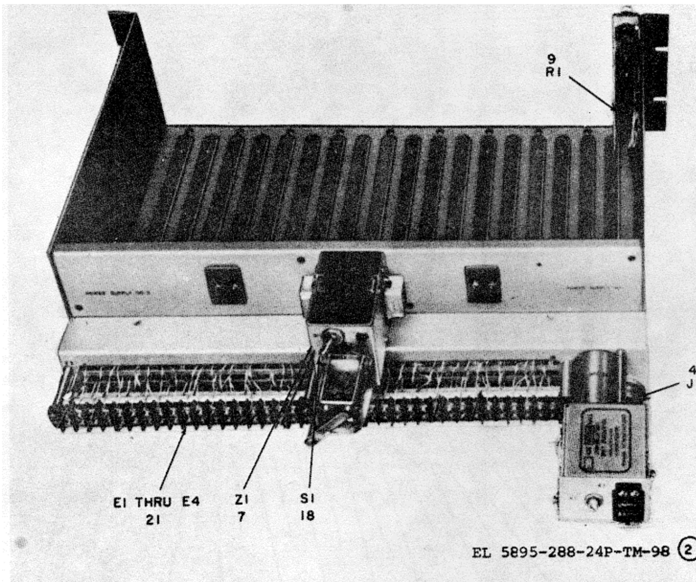
Figure 98. Tone Converter Shelf No. 1, Type 222, Model 5 (Sheet 2 of 2) 267
