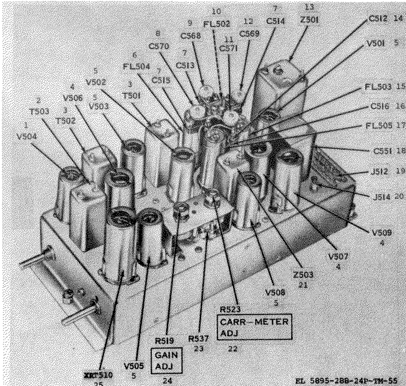
Figure 55. IF Subchassis, Mod 1, Order No. 363- Phila-54 and All IF Subchassis on Order No. 14-Phila-56, Top View
