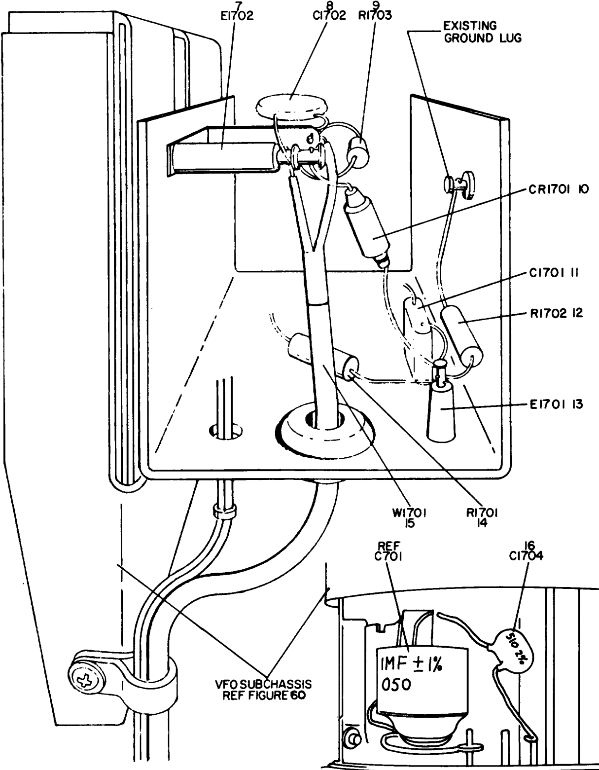
Figure 63. Radio Receiver Modification (Sheet 2 of 3)
