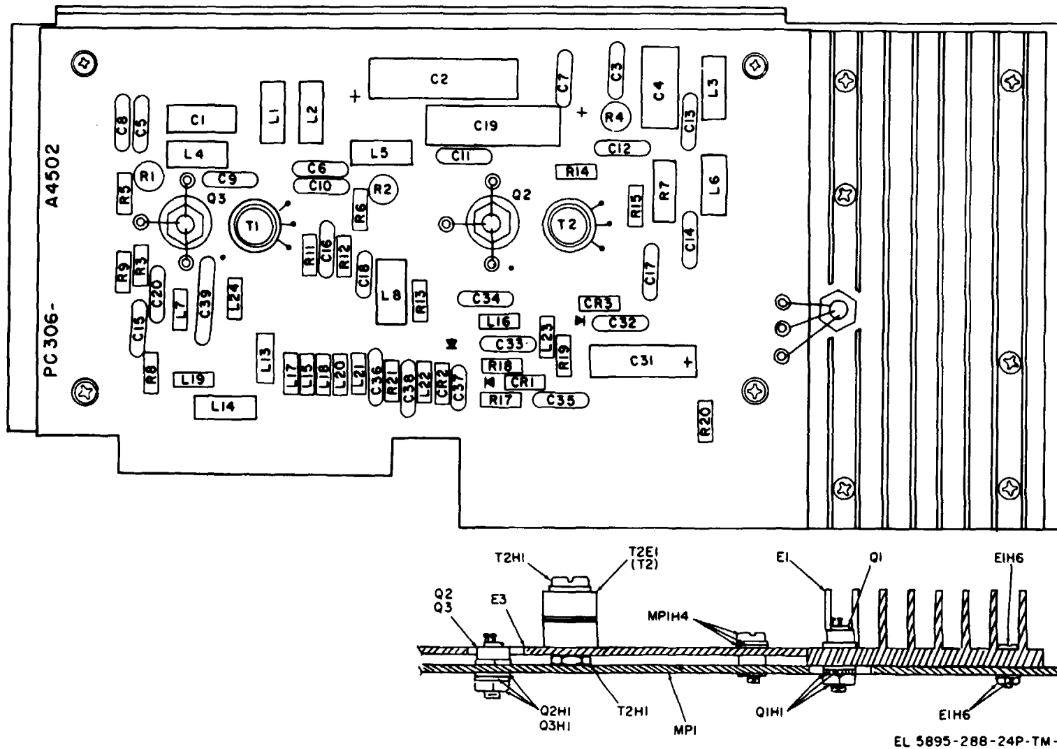
Figure 20. Radio Frequency Output Circuit Card Z115
