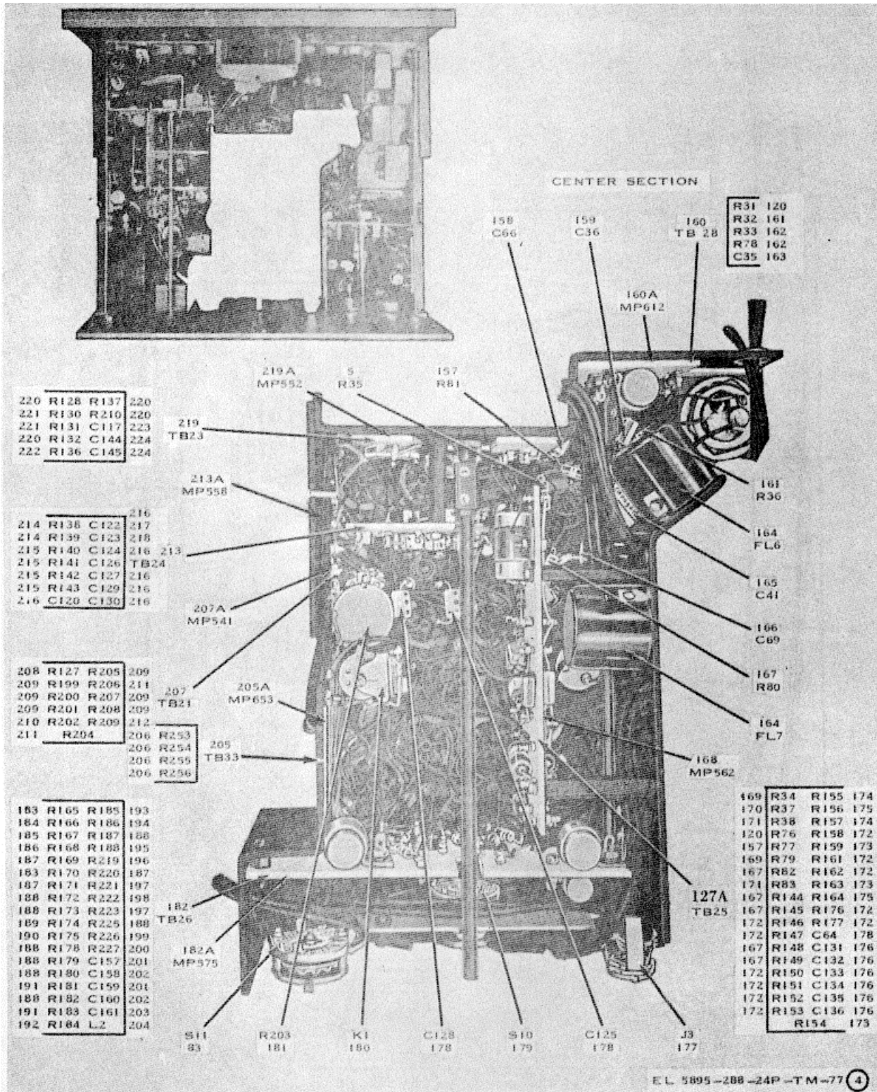
Figure 77. Converter Drawer Assembly, Bottom View (Sheet 4 of 4)
