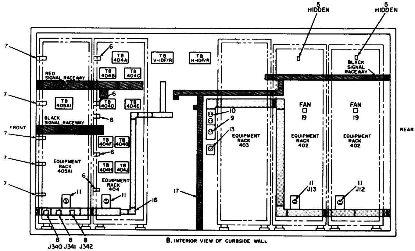
Figure 4. Electrical Equipment Shelter (Sheet 4 of 4)
