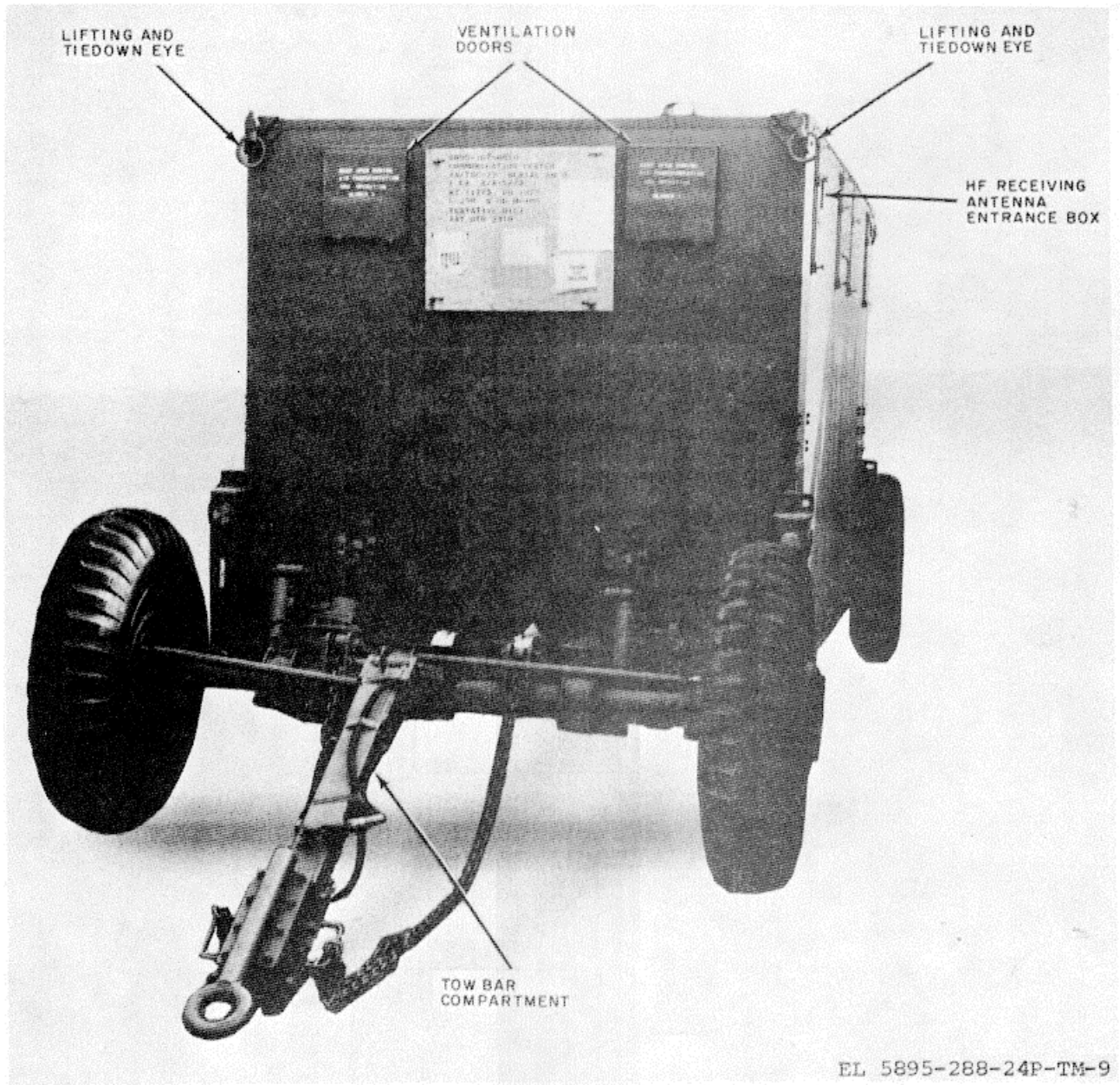
Figure 9. Transportable Shelter Dolly Set Lift
