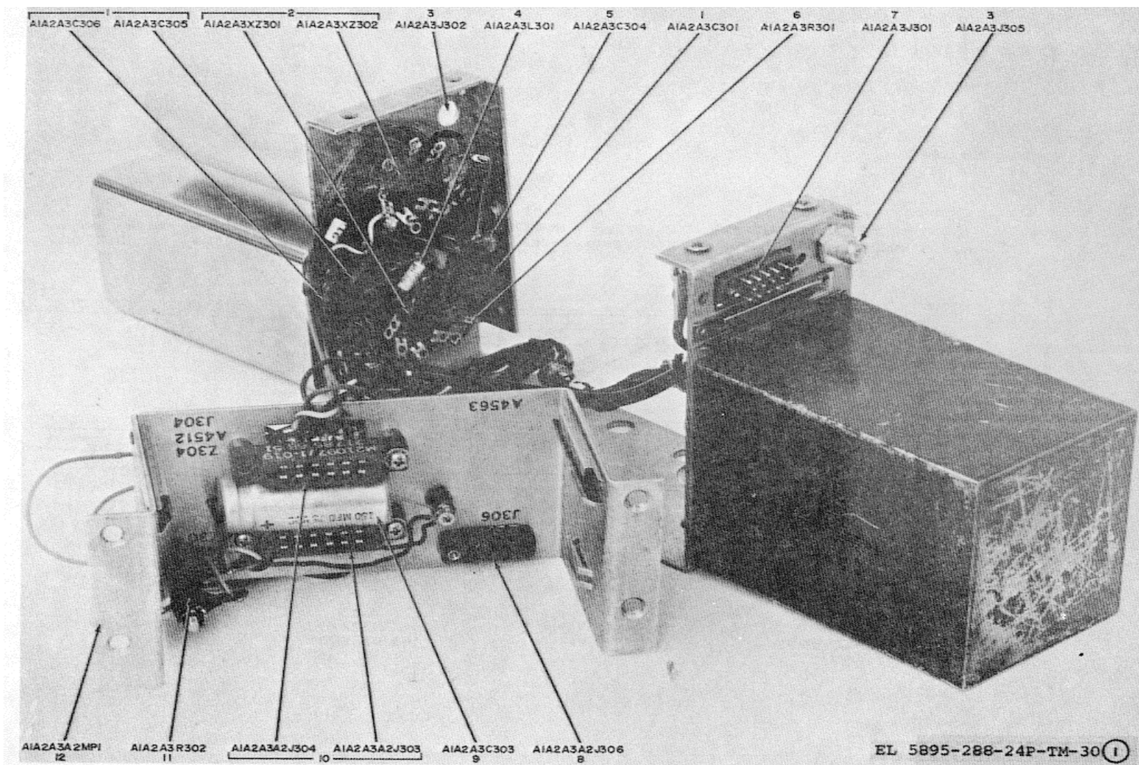
Figure 30. Power Supply (Sheet 1 of 2)
