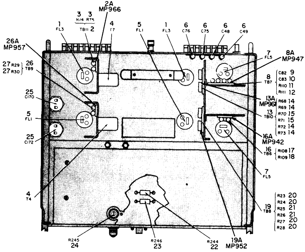
Figure 80. Converter Base Assembly, Top View
