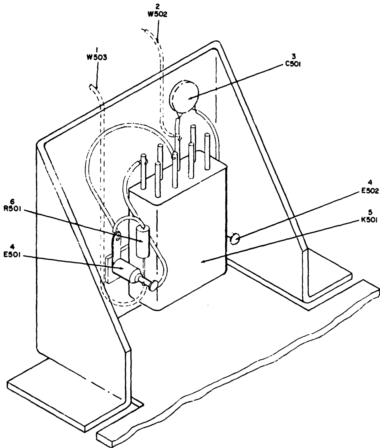
Figure 87. 100 XHz Oscillator Modification
