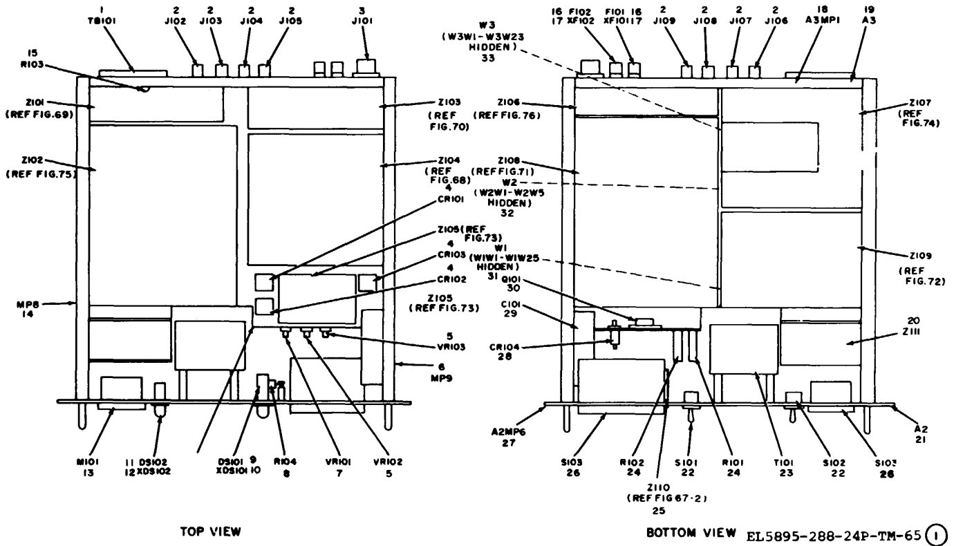
Figure 65. Main Chassis Assembly and Z110 (Sheet 1 of 2)
