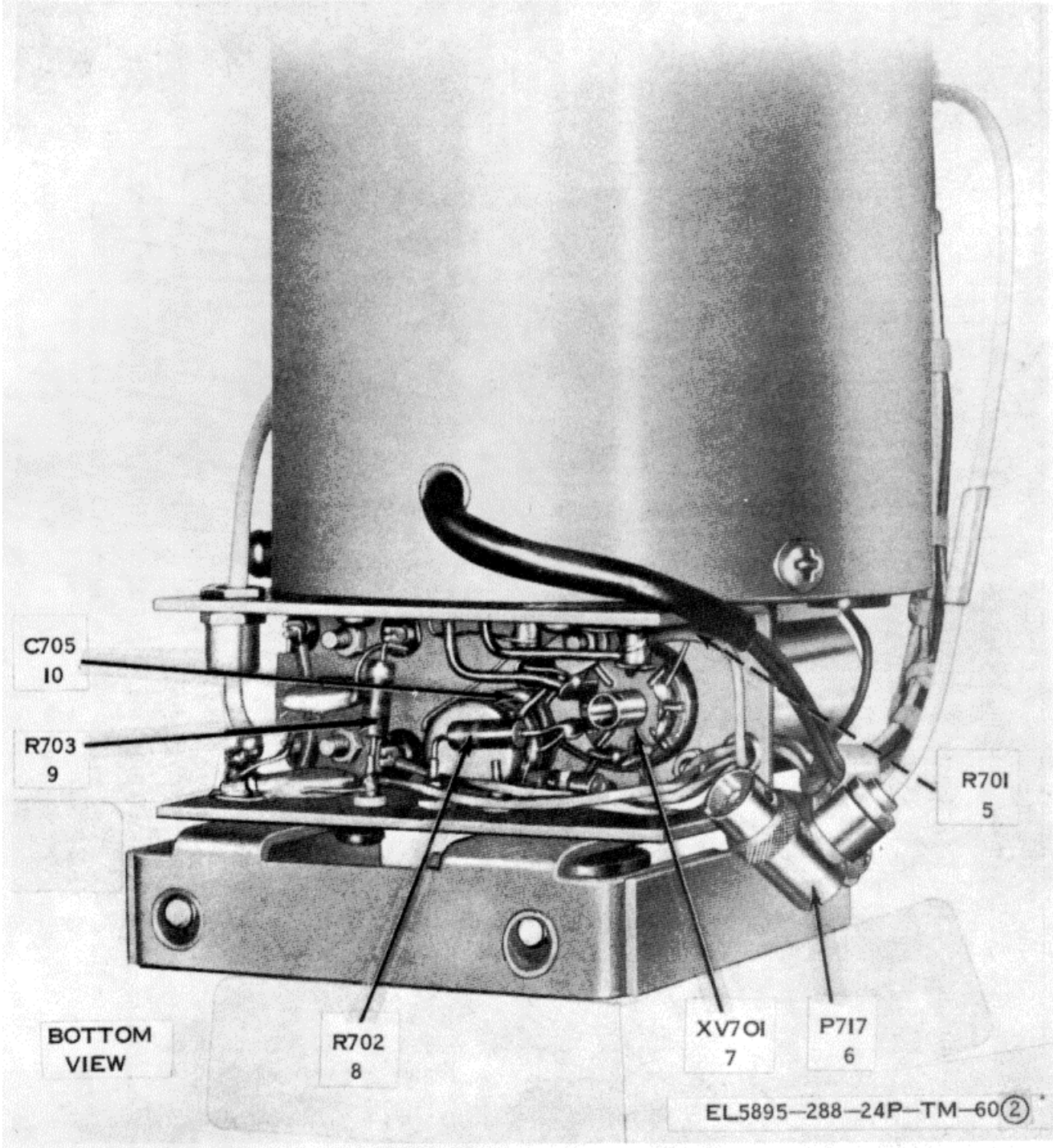
Figure 60. Radio Frequency Oscillator A1A6 (Sheet 2 of 2)
