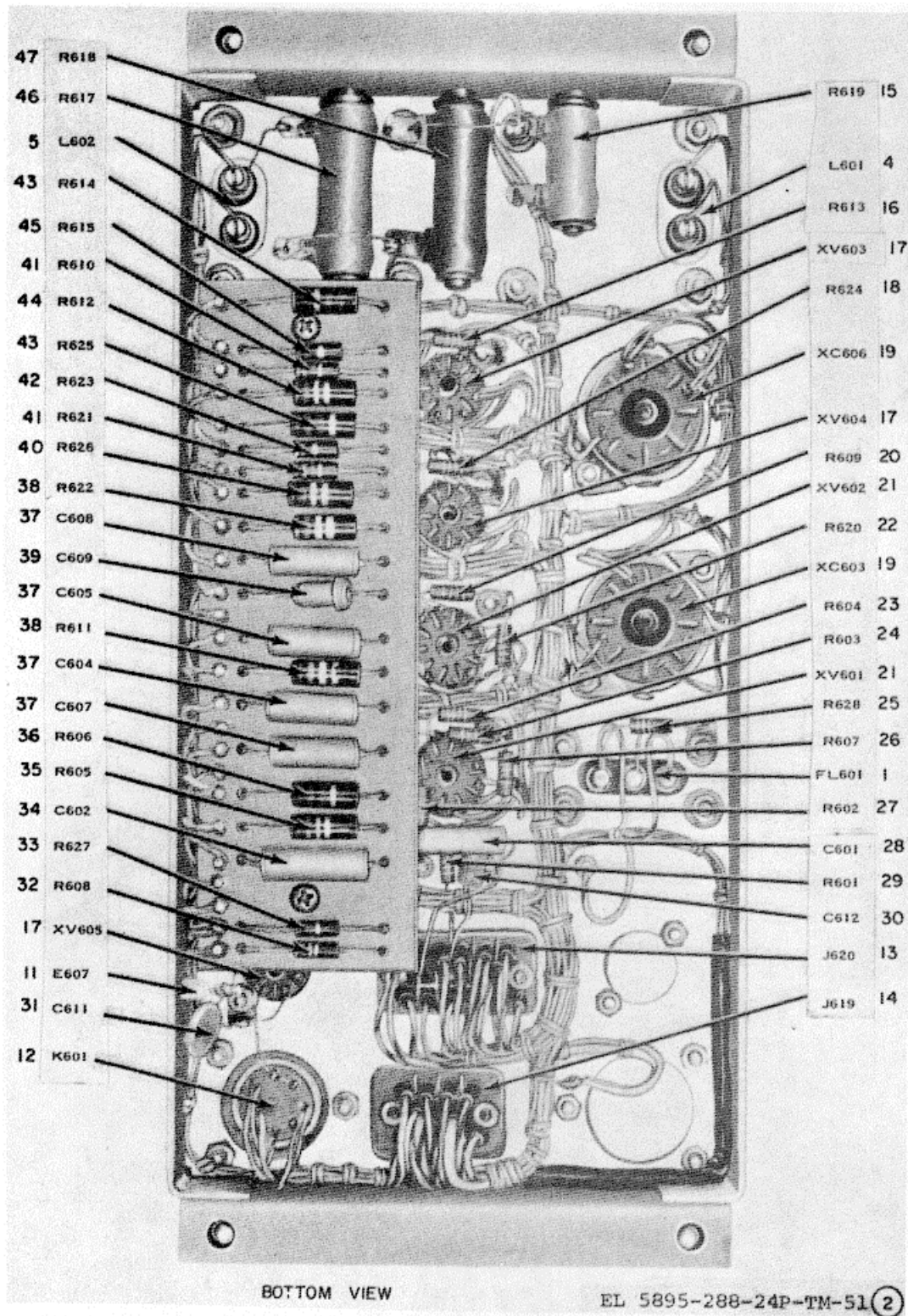
Figure 51. Audio Assembly A1A2 (Sheet 2 of 2)
