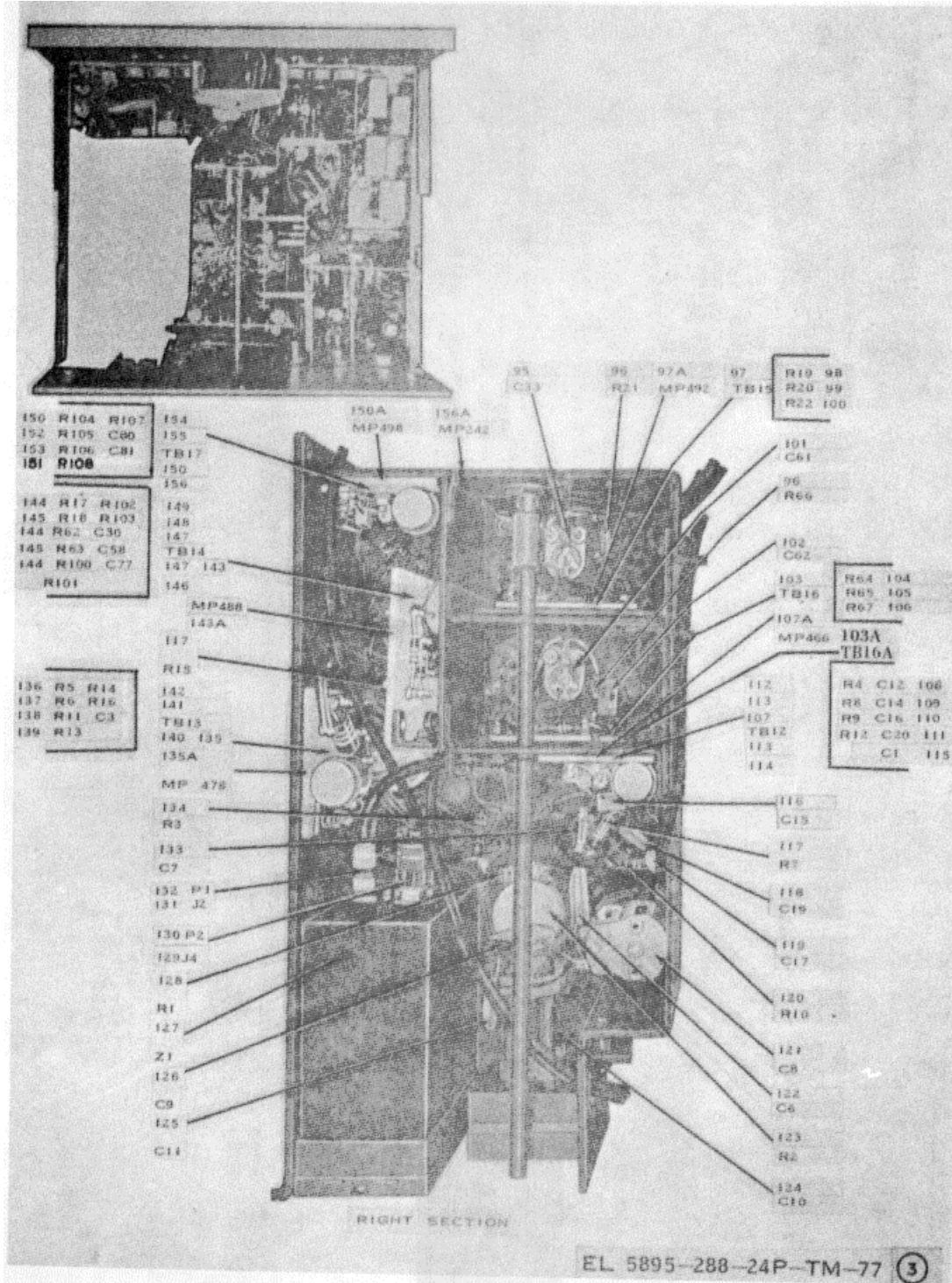
Figure 77. Converter Drawer Assembly, Bottom View (Sheet 3 of 4)
