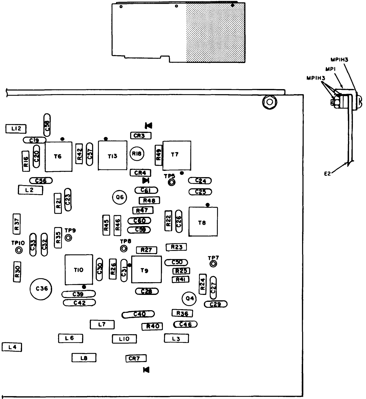
Figure 18. Mixer Divider Circuit Card Z106 (Sheet 2 of 2)
